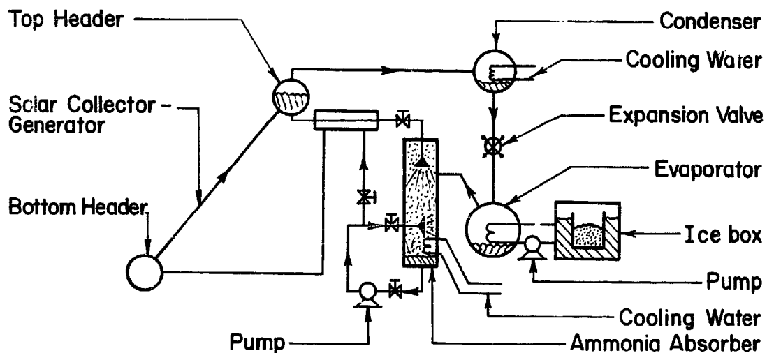
Fig.2.9- Solar Ice Maker Built at the University of Florida by FARBER (1970)
