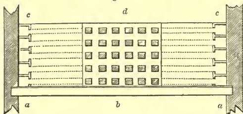
PART SECTION OF PIGEON-HOUSE—SCALE, \frac{1}{8} INCH TO THE FOOT.
