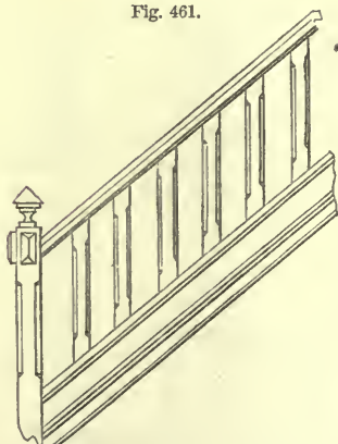
ELEVATION OF BALUSTERS FOR FARMHOUSE.
