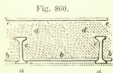
FIREPROOF FLOORING—SCALE, \frac{1}{2} INCH TO THE FOOT.
