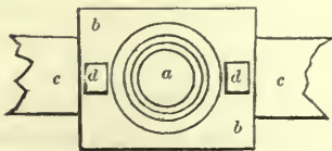
PLAN OF UPPER END OF COLUMN—SCALE, \frac{3}{4} INCH TO THE FOOT.
