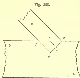
JOINT OF FOOT OF RAFTER WITH TIE-BEAM—SCALE, 1 INCH TO THE FOOT.
