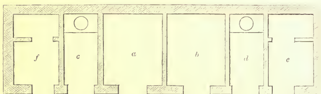
FIG. 136. ALTERNATIVE PLAN OF OUTHOUSES FOR DOUBLE DETACHED COTTAGES—SCALE IN FIG. 132.
