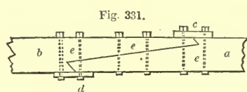
SCARF JOINT—SCALE, \frac{1}{4} INCH TO THE FOOT.
