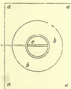
PLAN OF CHIMNEY-HOPPER AND BEARER.
