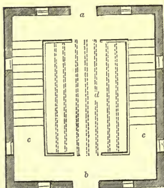
GROUND-PLAN OF AMERICAN POULTRY-HOUSE— SCALE, \frac{1}{2} INCH TO THE FOOT.
