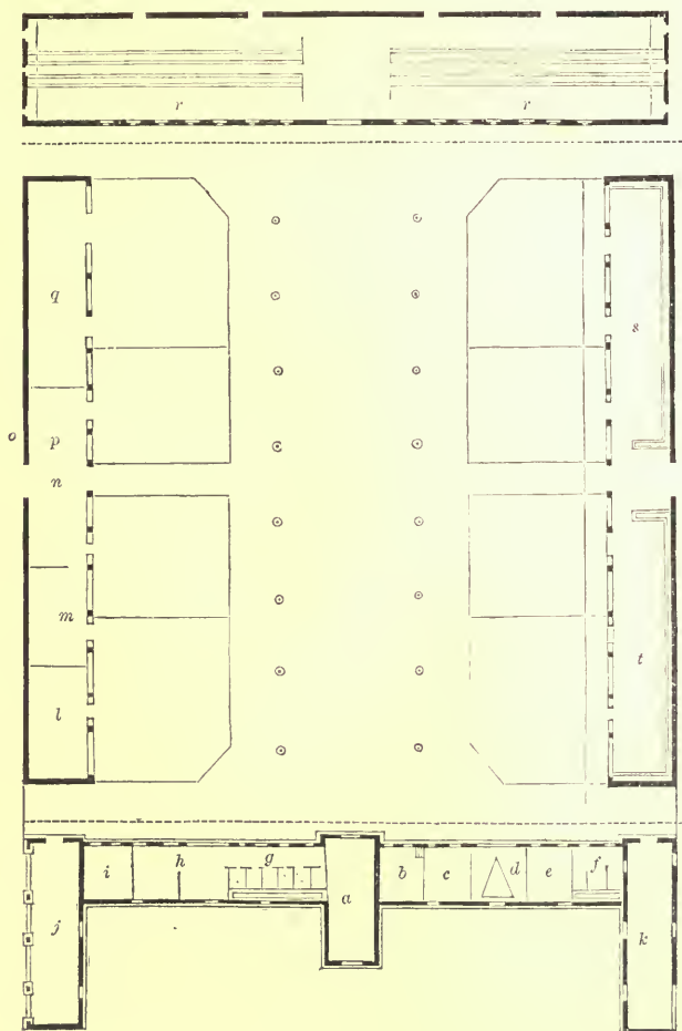
PLAN OF THE IMPERIAL FARM-STEADING AT VINCENNES.
