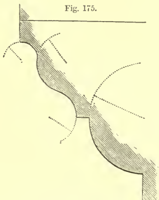
MOULDINGS TO CHIMNEY-CAP.
