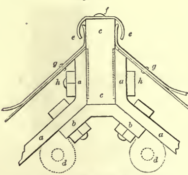
JOINING RAFTERS OF TRUSS FOR ZINC COVERING.
