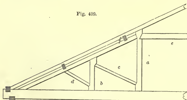
TRUSS WITH TWO QUEEN-POSTS FOR 47-FOOT SPAN—SCALE, \frac{1}{8} INCH TO THE FOOT.
