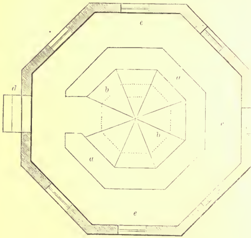
PLAN OF POULTRY-HOUSE—SCALE, \frac{1}{8} INCH TO THE FOOT.
