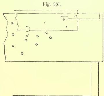
ELEVATION OF PART OF JOINER'S BENCH.
