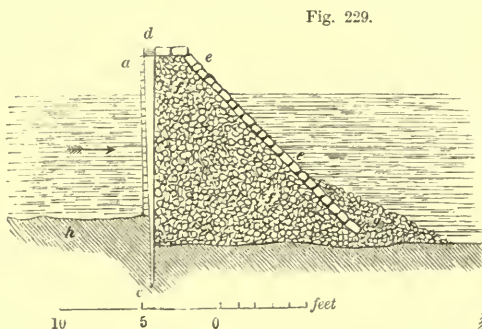
EMBANKMENT FOR A WATER RESERVOIR.
