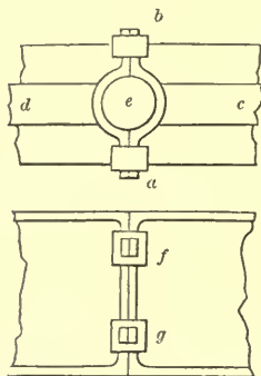
JUNCTION OF GIRDERS—SCALE, \frac{1}{2} INCH TO THE FOOT.
