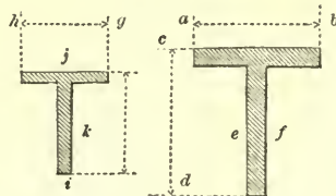
SECTION OF WROUGHT-IRON RAFTERS.
