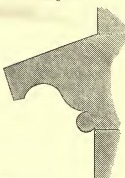
STRING-COURSE—SCALE, \frac{1}{8} FULL SIZE.
