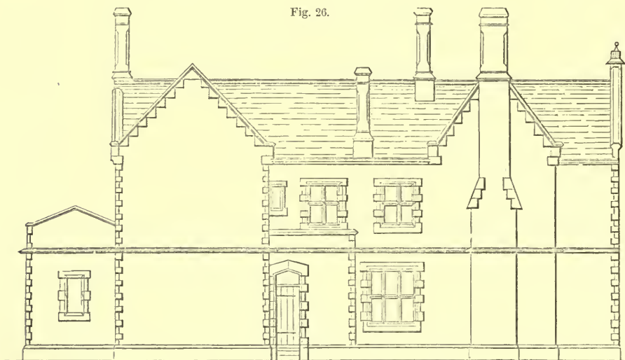
SIDE ELEVATION OF FARMHOUSE—SCALE IN PLATE XVIII.
