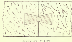
JOGGED JOINT
