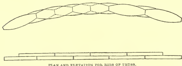
PLAN AND ELEVATION FOR RIBS OF TRUSS.
