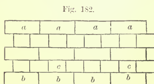
Fig. 182. OLD ENGLISH BRICK BOND.—SCALE, \frac{1}{2} INCH TO THE FOOT.
