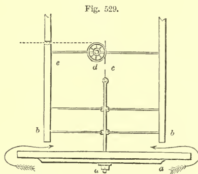
SECTION OF VENTILATOR WITH SUSPENDED VALVE.
