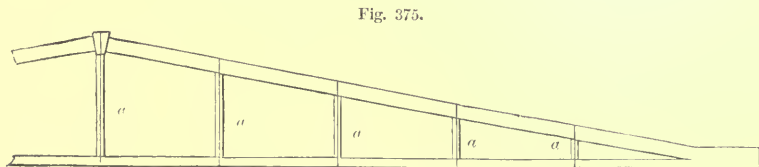
BOW-AND-STRING RAFTER—SCALE, \frac{1}{2} INCH TO THE FOOT.
