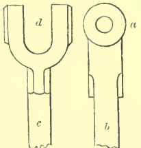
TERMINATION OF STRUTS AND TIE-BOLTS.
