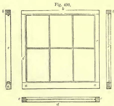
ELEVATION AND SECTION OF SASH-FRAME OF WINDOW.
