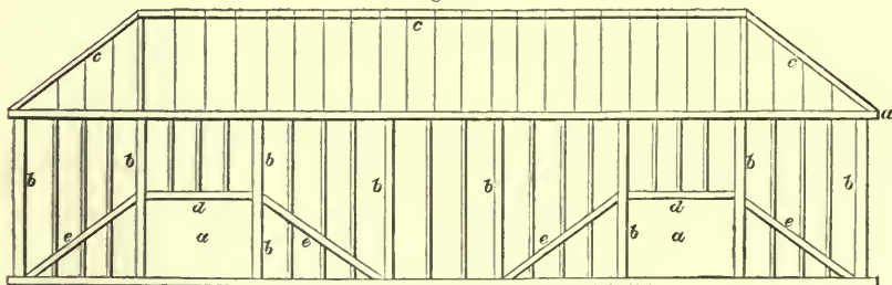
SIDE ELEVATION OF TIMBERS OF SHELTER-SHED.
