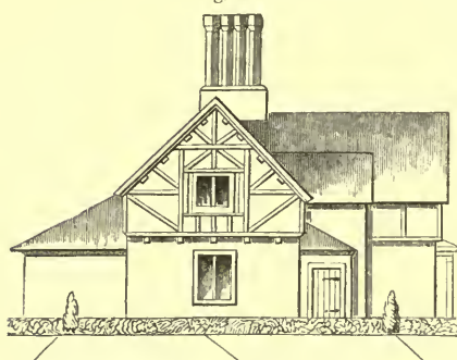
ELEVATION OF SMALL TWO-STORYED DOUBLE COTTAGES.
