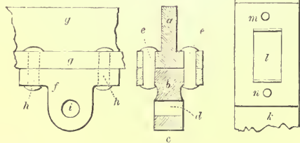
RIVETING STRUTS TO RAFTERS.
