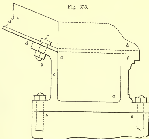
CAST-IRON GUTTER—SCALE IN FIG. 657.
