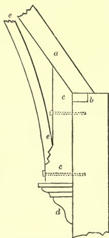
DETAIL OF PART OF ROOF-TRUSS —SCALE, \frac{1}{2} INCH TO THE FOOT.
