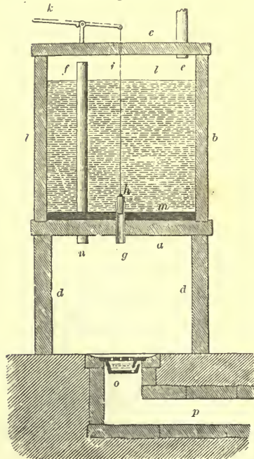
A RAIN-WATER CISTERN.
