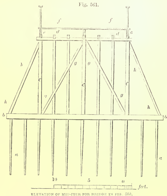
ELEVATION OF MID-TIER FOR BRIDGE IN FIG. 560.
