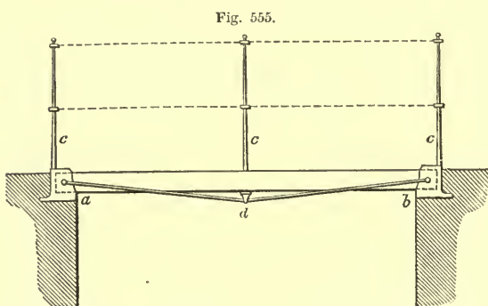
TRUSSED-BEAM BRIDGE, SPAN 8 FEET—SCALE, \frac{1}{2} INCH TO THE FOOT.
