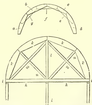
CENTRES FOR STONE CIRCULAR ARCHES—SCALE, \frac{1}{2} INCH TO THE FOOT.
