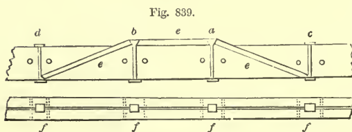
TRUSSED BEAM.
