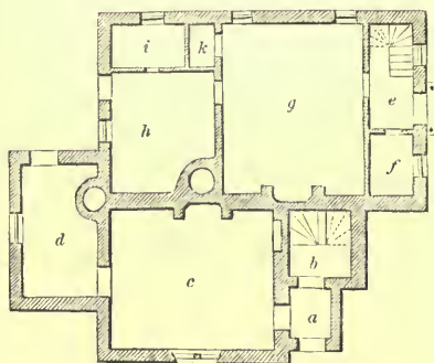
SMALL TWO-STOREYED DOUBLE COTTAGES.
