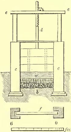
WOODEN SLUICE IN STONE GROOVES.
