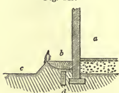
SECTION OF THE FOUNDATION OF A HIND'S HOUSE.
