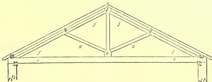
KING-POST ROOF—SCALE IN FIG. 990.
