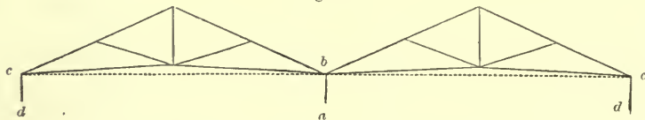
SKELETON TRUSS OF DOUBLE-SPAN ROOF—SCALE IN FIG. 657.
