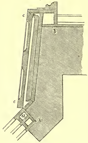
PLAN OF BAY WINDOW SHUTTERS—SCALE IN FIG. 516.
