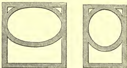
SECTIONS OF DOULTON'S VENTILATING CHIMNEY-TUBE.
