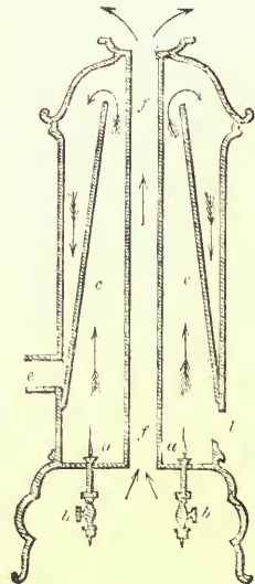
RICKETT'S GAS-STOVE.
