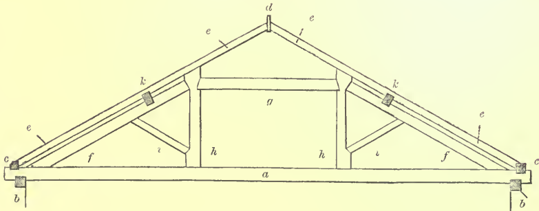
QUEEN-POST TRUSS FOR 30 TO 45 FEET SPAN—SCALE, \frac{1}{8} INCH TO THE FOOT.
