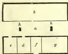
PLAN OF UPPER STOREY OF AMERICAN BARN.
