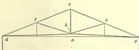
SKELETON TRUSS FOR AN IRON ROOF OF 18-FOOT SPAN.
