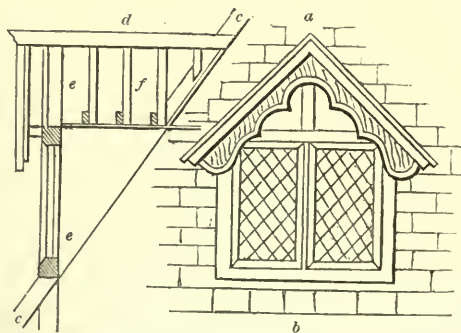
ELEVATION AND SECTION OF DORMER WINDOW—SCALE, \frac{1}{4} INCH TO THE FOOT.
