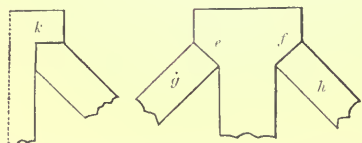
JOINTS OF STRUTS AND RAFTERS WITH HEADS AND FEET OF KING-POSTS AND QUEEN-POSTS—SCALE, \frac{1}{2} INCH TO THE FOOT.
