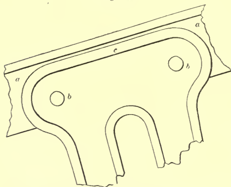
UPPER TERMINATION OF STRUT—SCALE IN FIG. 657.
