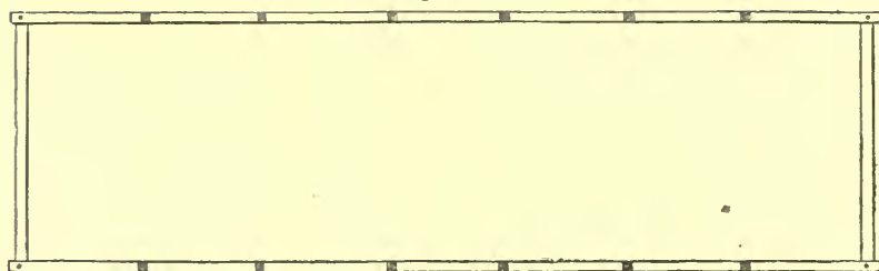
0 10 30 50 feet. PLAN OF BALK FOUNDATIONS OF SHELTER-SHED.
