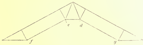
SKELETON TRUSS FOR SHED.
