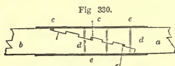
SCARF JOINT—SCALE, \frac{1}{4} INCH TO THE FOOT.
