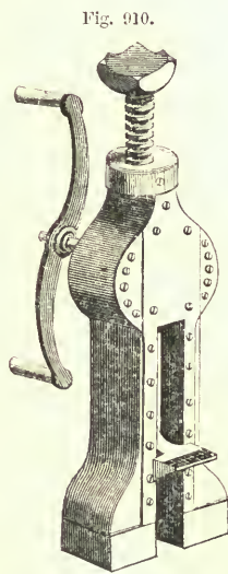
HALLEY'S PATENT LIFTING-JACK.
