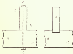
JOINING OF BEAMS CROSSING EACH OTHER AT RIGHT ANGLES—SCALE, \frac{1}{2} INCH TO THE FOOT.
