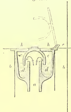
BELL TRAP.
