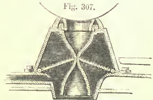
JENNINGS'S WATER-CLOSET—TUBE CLOSED.
