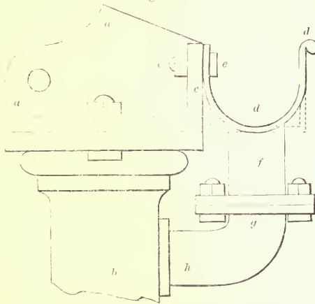
CAST-IRON GUTTER, LEADING WATER TO THE COLUMN— SCALE IN FIG. 657.
