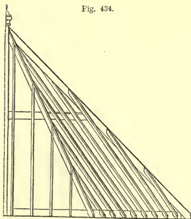
ELEVATION OF HEXAGONAL ROOF—SCALE, \frac{1}{8} INCH TO THE FOOT.
