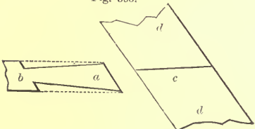
JOINT OF COLLAR-BEAM WITH RAFTER—SCALE, \frac{1}{2} INCH TO THE FOOT.
