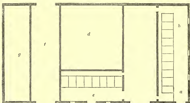
PLAN OF DUTCH BARN—SCALE AS IN FIG. 963.
