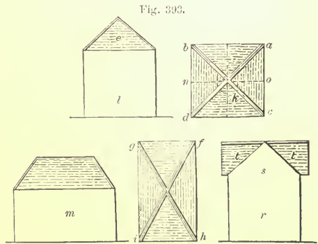
PAVILION ROOF.
