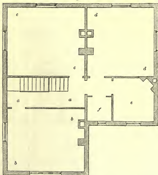
CHAMBER-FLOOR PLAN OF A THIRD-CLASS FARMHOUSE—SCALE, \frac{3}{16} OF AN INCH TO THE FOOT.
