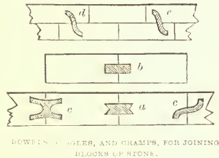
DOWELS, JOGGLES, AND CRAMPS, FOR JOINING BLOCKS OF STONE.
