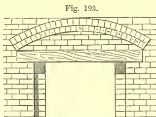
CURVED ARCH AND LINTEL.
