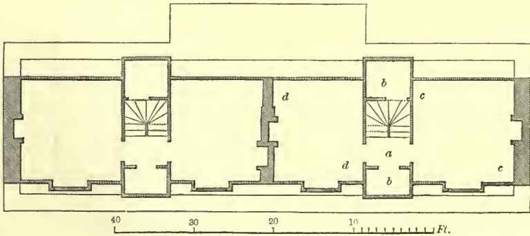
CHAMBER-FLOOR PLAN OF FIG. 103
