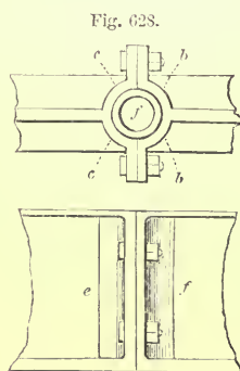
JUNCTION OF GIRDERS WITH CIRCULAR NECK TO COLUMNS—SCALE, \frac{1}{2} INCH TO THE FOOT.
