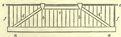
QUEEN-POST TRUSS FOR BRIDGE—SCALE, \frac{1}{2} INCH TO THE FOOT.
