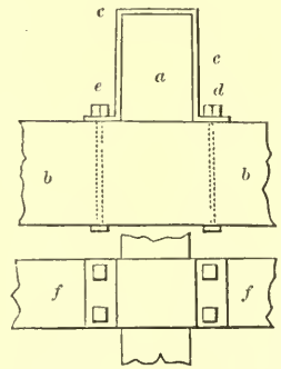
IRON SADDLE FOR JOINING BEAMS CROSSING AT RIGHT ANGLES—SCALE, \frac{1}{2} INCH TO THE FOOT.
