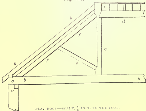
FLAT ROOF—SCALE, \frac{1}{4} INCH TO THE FOOT.
