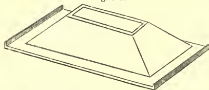
CAST-IRON CHIMNEY-HOPPER AND BEARER COMBINED.
