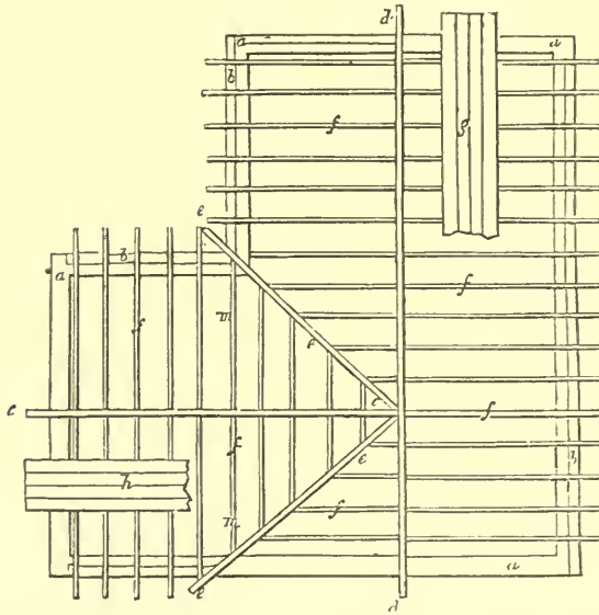
TIMBER OF A ROOF MEETING AT RIGHT ANGLES (PLAN)—SCALE, \frac{1}{8} INCH TO THE FOOT.
