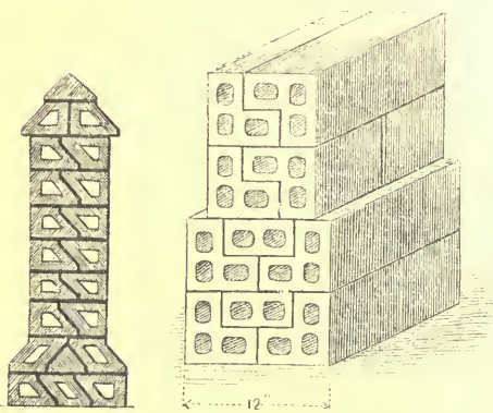
SECTION OF 12-INCH HOLLOW WALL
