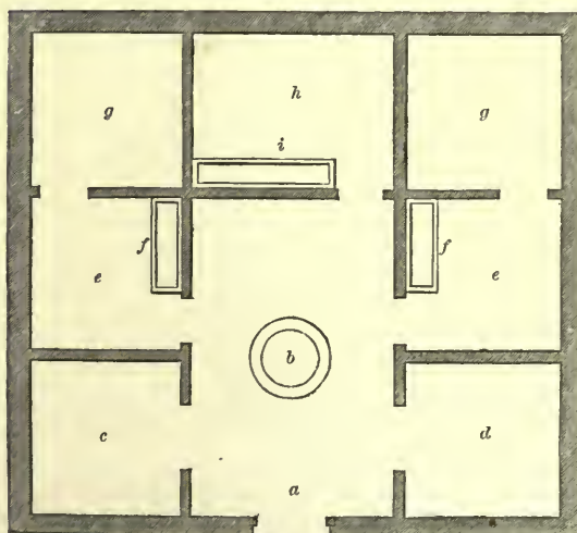
PLAN OF DETACHED PIGGERY—SCALE, \frac{1}{8} INCH TO THE FOOT.
