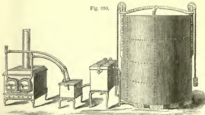
PERSPECTIVE VIEW OF MESSRS BRIDGES AND AUBURY'S GAS-MAKING APPARATUS.
