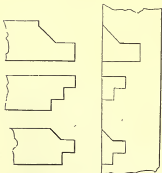
TUSE JOINTS—SCALE, \frac{1}{2} INCH TO THE FOOT.
