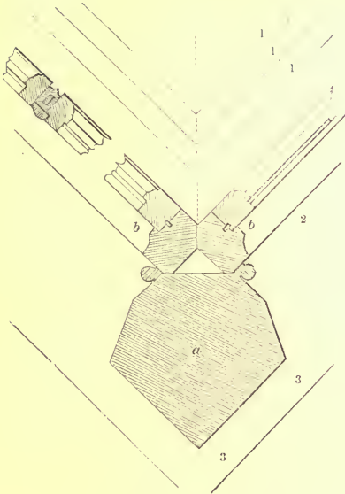
PART SECTIONAL PLAN OF WINDOW—SCALE, 1 INCH TO THE FOOT.
