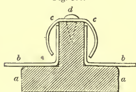
ATTACHING SHEETS OF ZINC TO WROUGHT-IRON RAFTERS.
