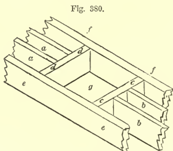
TRIMMING-JOISTS—SCALE, \frac{1}{2} INCH TO THE FOOT.
