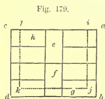
Fig. 179. PLAN OF SECOND COURSE OF FOOTINGS.—SCALE, \frac{1}{2} INCH TO THE FOOT.
