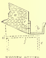
WOODEN GUTTER.
