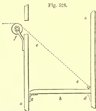
SECTION OF VENTILATOR WITH HINGED VALVE.
