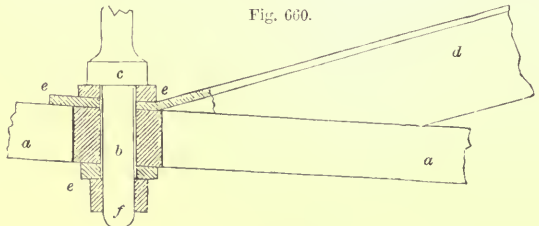
JOINING OF FOOT OF QUEEN-BOLT WITH STRUT.
