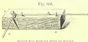
BLOCK FOR MAKING EYES IN WIRES.
