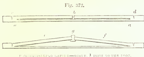
BOW-AND-STRING RAFTER—SCALE, \frac{1}{4} INCH TO THE FOOT.
