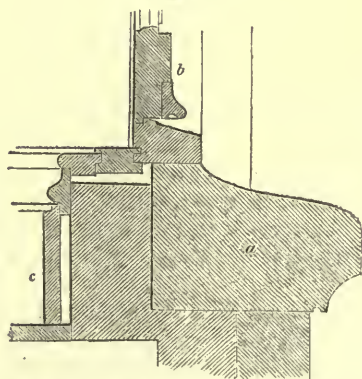
PART SECTION OF BASE OF BAY WINDOW—SCALE, 1 INCH TO THE FOOT.
