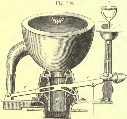
SECTION OF JENNINGS'S WATER-CLOSET—TUBE OPEN.
