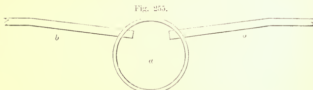
SECTION OF CROSS-CULVERT AND UNDER-DRAIN
