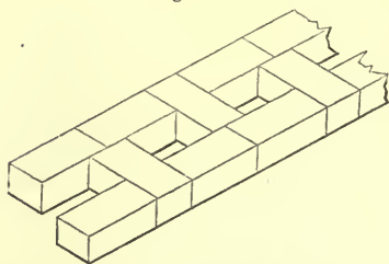
14-INCH HOLLOW WALL—SCALE, \frac{1}{2} INCH TO THE FOOT.
