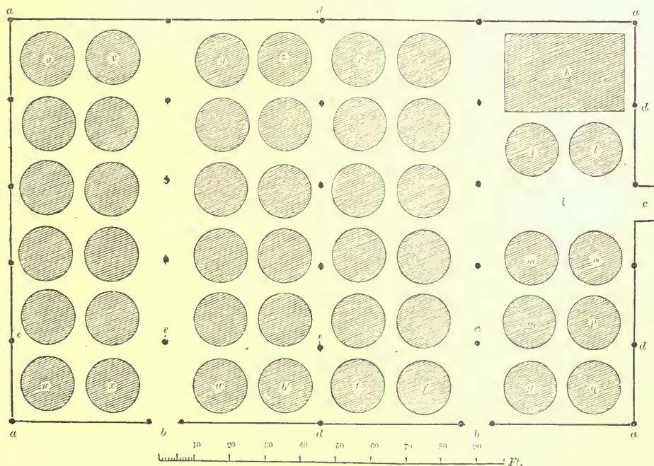
GROUND-PLAN OF A COVERED STACKYARD.
