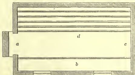
PLAN OF POULTRY-HOUSE—SCALE, \frac{1}{2} INCH TO THE FOOT.
