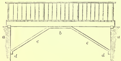
BRIDGE FOR 14-FEET SPAN, WITH STRUTS—SCALE, \frac{1}{8} INCH TO THE FOOT.
