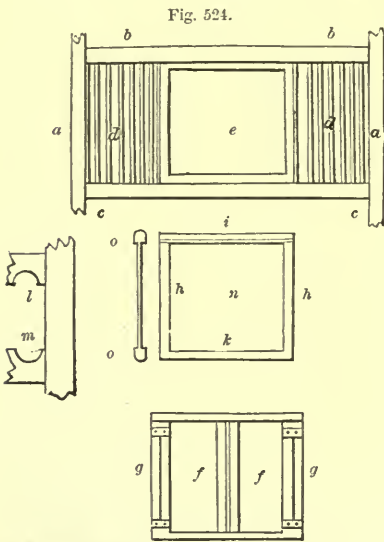
FIG. 524. FITTINGS OF HEAD OF STALL WITH FEEDING-PASSAGE— SCALE, \frac{1}{2} INCH TO THE FOOT.
