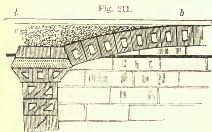
FIG. 211. SECTION AND DETAILS IN ROBERTS' HOLLOW BRICKS.
