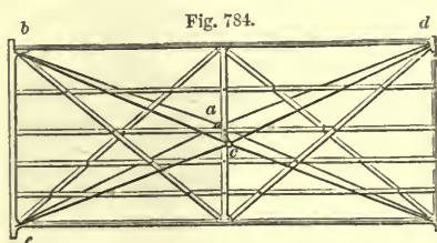
IRON FIELD-GATE ON THE TENSION PRINCIPLE.
