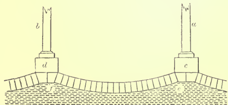
INVERTED ARCHES FOR FOUNDATIONS—SCALE, \frac{1}{2} INCH TO THE FOOT.
