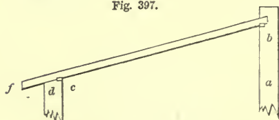
LEAN-TO ROOF, &amp;c., 12-FOOT SPAN—SCALE, ½ INCH TO THE FOOT.
