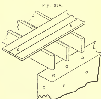
SINGLE FLOORING—SCALE, \frac{1}{2} INCH TO THE FOOT.
