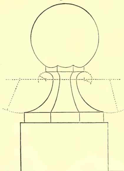
ELEVATION OF STONE FINIAL—SCALE, \frac{1}{8} FULL SIZE.
