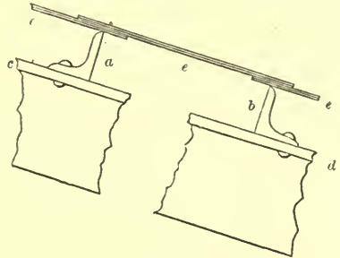
FIXING OF SLATES WITH IRON ROOF—SCALE IN FIG. 657.
