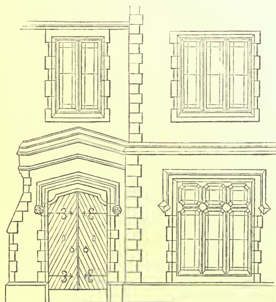
ENLARGED VIEW OF PART OF FRONT ELEVATION IN FIG. 47—SCALE, \frac{1}{8} OF AN INCH TO THE FOOT.
