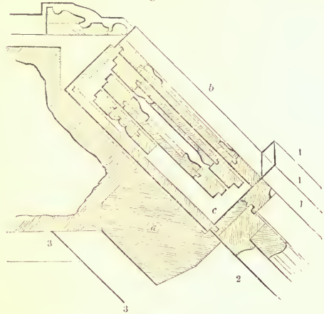
PLAN OF WINDOW SHUTTER—SCALE, 1 INCH TO THE FOOT.
