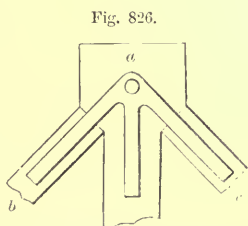
IRON STRAP FOR HEAD OF KING-POST AND BRACES—SCALE, \frac{1}{4} INCH TO THE FOOT.
