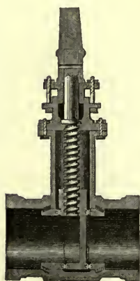
JENNING'S SLUICE-VALVE.
