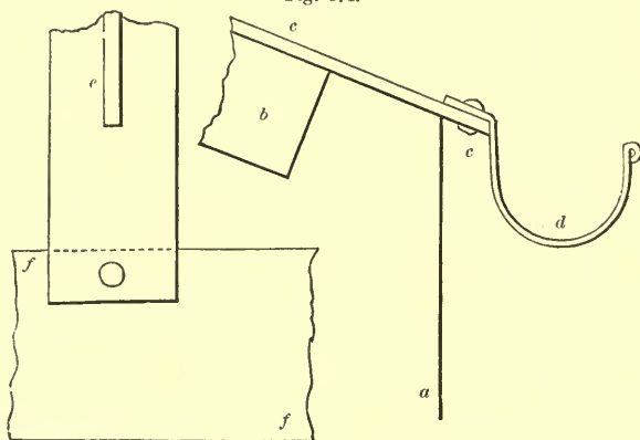
GUTTER OF IRON ROOF—SCALE IN FIG. 657.
