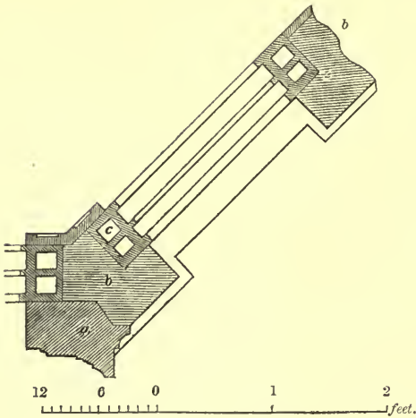
PART PLAN OF BAY WINDOW OF HOUSE IN FIG. 63—SCALE, 1 INCH TO THE FOOT.
