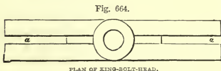
PLAN OF KING-BOLT-HEAD.
