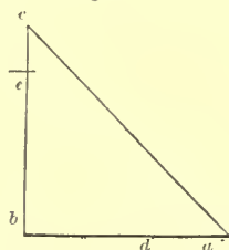
TEMPLATE FOR MARKING OUT STEPS.
