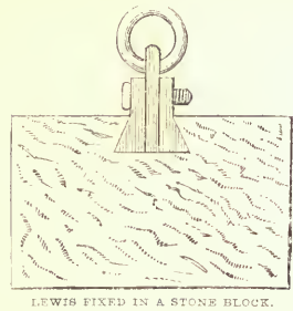
LEWIS FIXED IN A STONE BLOCK.
