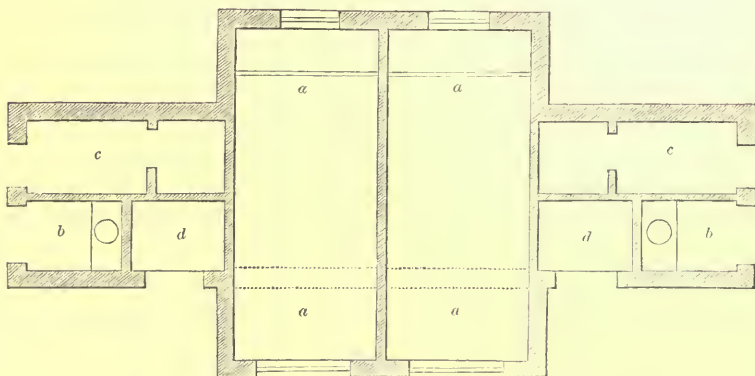
SECOND ALTERNATIVE PLAN OF OUTHOUSES FOR DOUBLE DETACHED COTTAGES—SCALE IN FIG. 132.
