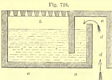
LOWE'S CAST-IRON TRAP.
