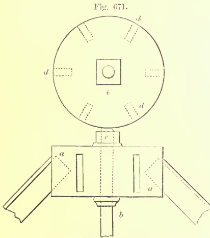
KING-BOLT AND HEAD—SHOE IN ELEVATION AND PLAN— SCALE, 1 INCH TO THE FOOT.
