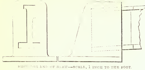
SHOT FOR END OF BEAM—SCALE, 1 INCH TO THE FOOT.
