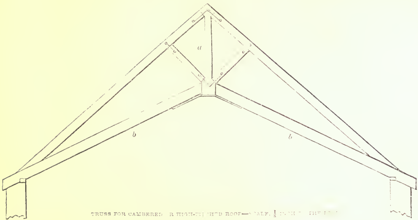
TRUSS FOR CAMBERED OR HIGH-CURVED ROOF—SCALE, \frac{1}{4} INCH TO THE FOOT.
