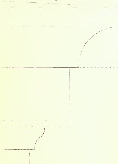
MOULDINGS OF WINDOW CORNICE—SCALE, \frac{1}{4} FULL SIZE.
