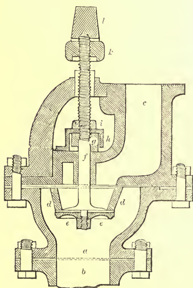
WHEATECROFT AND SMITH'S HYDRANT
