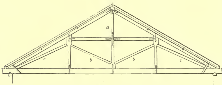
TRUSS FOR A 30-FOOT SPAN—SCALE, \frac{1}{8} INCH TO THE FOOT.
