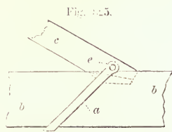
IRON STRAP FOR FOOT OF RAFTER AND TIE BEAM—SCALE, \frac{1}{4} INCH TO THE FOOT.
