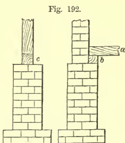
BEARING WALLS.
