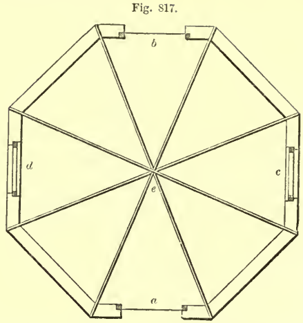
PLAN OF OCTAGONAL SHED—SCALE, \frac{1}{8} INCH TO THE FOOT.
