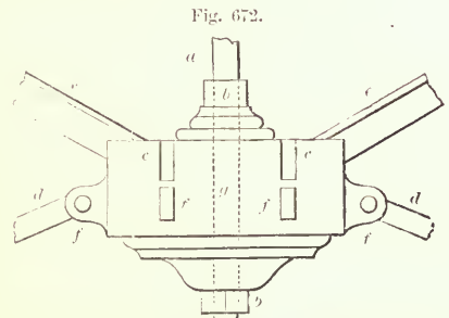
SHOE FOR RECEIVING THE ENDS OF RAFTERS AND UPPER ENDS OF TIE-BOLTS—SCALE, 1 INCH TO THE FOOT.
