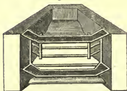
PERSPECTIVE VIEW OF PIERCE'S COTTAGE FIRE-LUMP GRATE.
