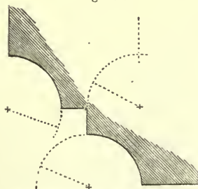
MOULDINGS OF JAMB AND MULLION OF DOORWAY—SCALE, \frac{1}{8} FULL SIZE
