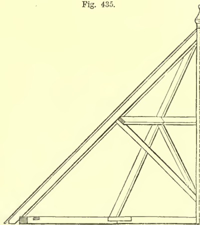
SECTION OF HEXAGONAL ROOF—SCALE, \frac{1}{8} INCH TO THE FOOT.
