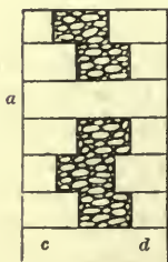
MODE OF BUILDING ASHLAR WALLS WITH “RUBBLE” FILLING-IN —SCALE, 1/4 INCH TO THE FOOT.
