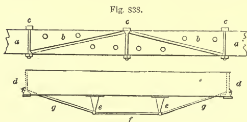
TRUSSED BEAM.
