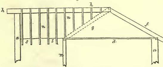
ELEVATION OF ROOF IN FIG. 413—SCALE, \frac{1}{8} INCH TO THE FOOT.
