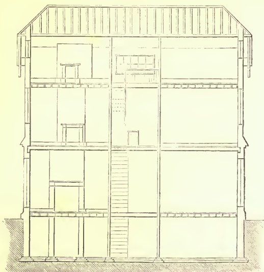
TRANSVERSE SECTION OF LARCH HOUSE—SCALE IN FIG. 47.
