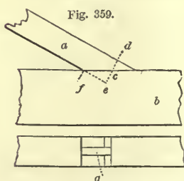
JOINING OF AN INCLINED WITH A HORIZONTAL BEAM—SCALE, \frac{1}{2} INCH TO THE FOOT.
