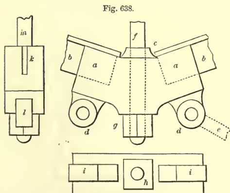
JUNCTION OF KING-BOLT, STRUTS, RAFTERS, AND TIE-RODS—SCALE IN FIG. 637.
