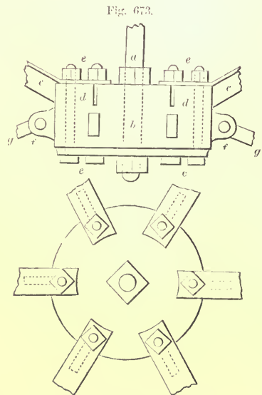
JUNCTION OF KING-BOLT, STRUTS, AND TIE BOLTS—SCALE, 1 INCH TO THE FOOT.
