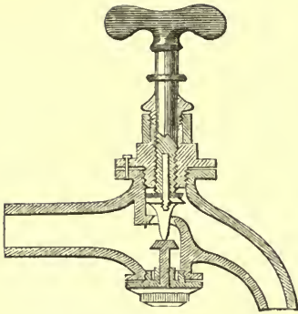
CHRIMES'S WATER-TAP.
