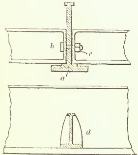
CONNECTION OF CROSS-BEAMS WITH GIRDERS—SCALE, \frac{1}{2} INCH TO THE FOOT.
