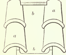
PEAKE'S RIDGE-TILES.
