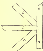
JOINING OF HIP-RAFTERS WITH RIDGE-POLE—SCALE, \frac{1}{4} INCH TO THE FOOT.
