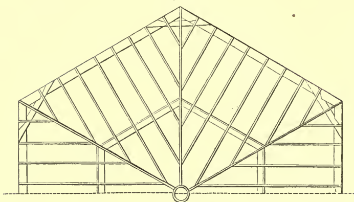
PLAN OF HEXAGONAL TRUSS—SCALE, \frac{1}{8} INCH TO THE FOOT.
