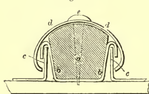
FIXING SHEETS OF ZINC TO WOODROLLS
