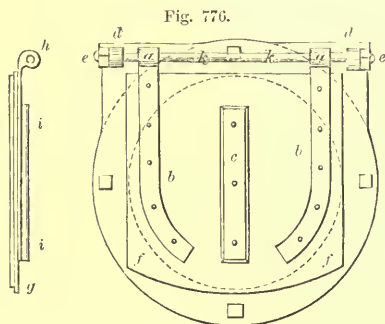
FRONT ELEVATION OF SLUICE-VALVE—SCALE, \frac{3}{4} INCH TO THE FOOT.
