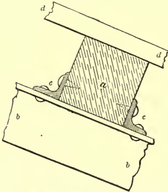
JUNCTION OF WOODEN PURLINS WITH IRON RAFTERS—SCALE IN FIG. 657.
