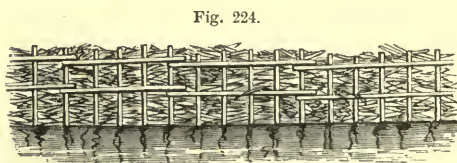
COMMON PILING FOR THE PROTECTION OF RIVER-BANKS.
