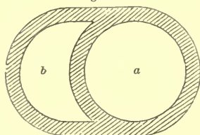
SECTIONAL PLAN OF CHIMNEY AND VENTILATING TUBE.
