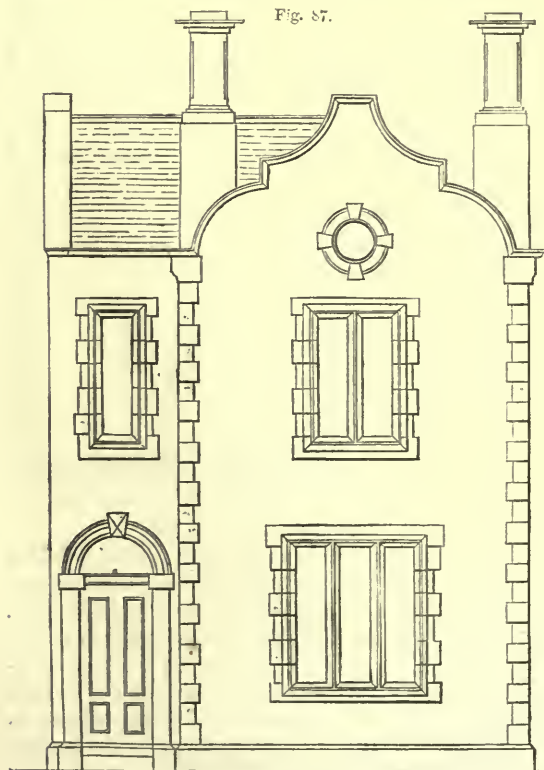
FRONT ELEVATION OF THE TWO-STOREYED COTTAGE IN FIG. 85.
