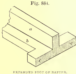
EXPANDED FOOT OF RAFTER.
