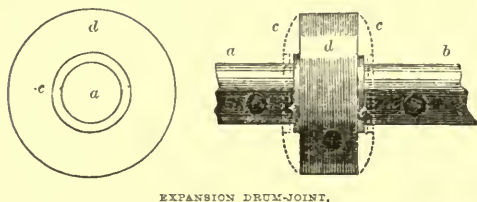
EXPANSION DRUM-JOINT.
