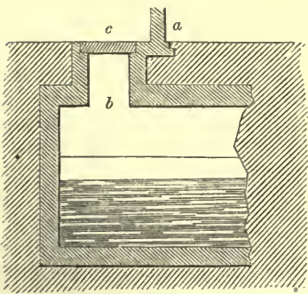
FLEMISH LIQUID-MANURE TANK.
