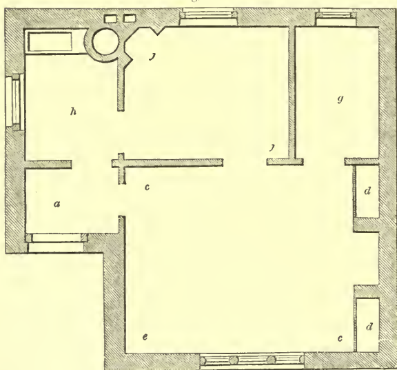
Fl. 11111 5 10 15 20 GROUND-PLAN OF SINGLE-STOREYED DETACHED COTTAGE.
