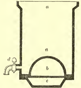
SECTION OF COMBINED CALDRON AND FURNACE.
