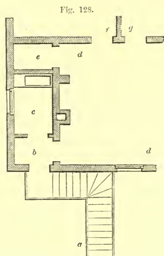
UPPER PLAN OF COMPOSITE COTTAGE APPLIED TO FIG. 119—SCALE IN FIG. 115.
