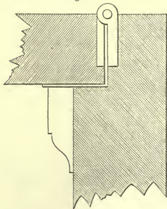
PLAN OF DOOR STOP (DOOR CLOSED).
