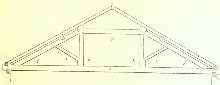
QUEEN-POST ROOF.—SCALE, \frac{1}{8} INCH TO THE FOOT.
