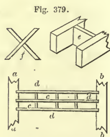
TRUSSING OF FLOORING BEAMS—SCALE, \frac{1}{2} INCH TO THE FOOT.
