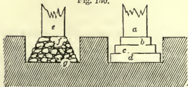
STONE FOOTINGS—SCALE, \frac{1}{2} INCH TO THE FOOT.
