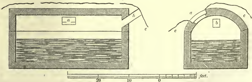
SECTION OF A FLEMISH LIQUID-MANURE TANK.
