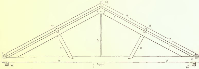
TRUSS FOR A 30-FOOT SPAN—SCALE, \frac{1}{8} INCH TO THE FOOT.
