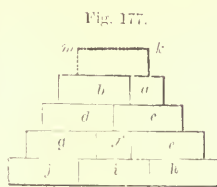
Fig. 177. SECTION OF A 14-INCH BRICK WALL.—SCALE, \frac{1}{2} INCH TO THE FOOT.
