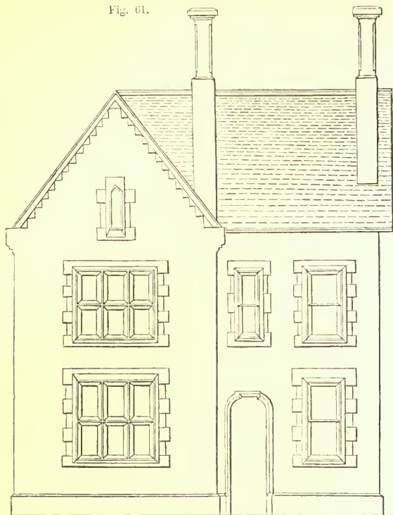
FRONT ELEVATION OF A THIRD-CLASS FARMHOUSE.—SCALE, \frac{1}{4} " = 1 FT. AN INCH TO THE FOOT
