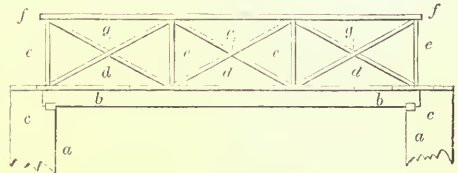
BEAM-BRIDGE FOR 15 FEET SPAN—SCALE, \frac{1}{8} INCH TO THE FOOT.
