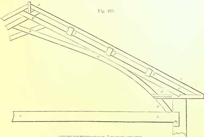
CURVED RIB-TRUSS—SCALE, \frac{1}{4} INCH TO THE FOOT.
