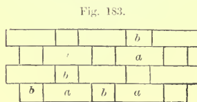
Fig. 183. FLEMISH BOND.—SCALE, \frac{1}{2} INCH TO THE FOOT.
