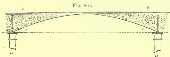
FIREPROOF FLOORS WITH WROUGHT-IRON BEAMS—SCALE, \frac{1}{4} INCH TO THE FOOT.
