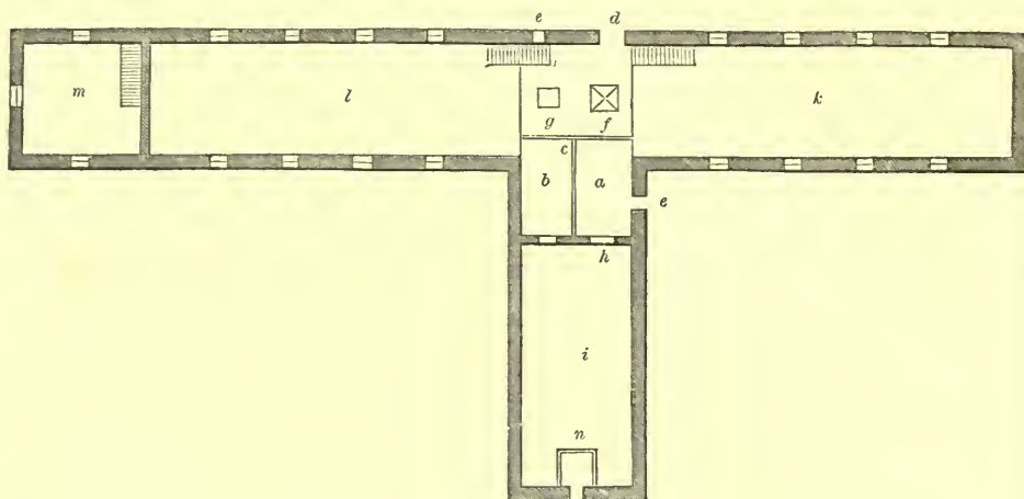
UPPER STOREY OF A STEADING FOR SUBURBIAL DAIRY FARMING.
