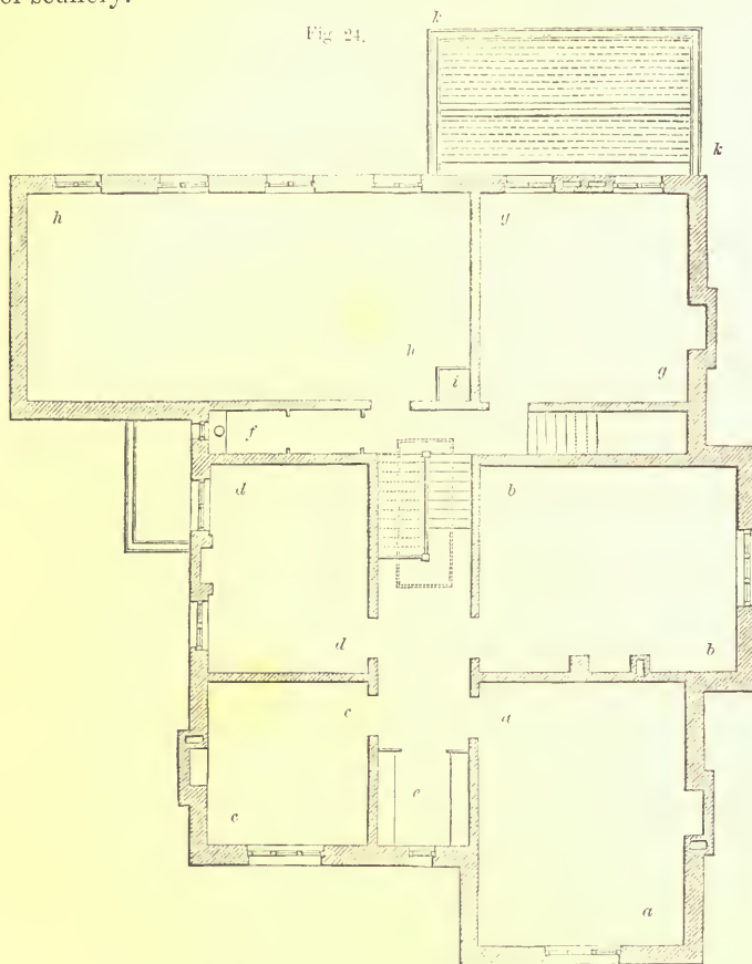
CHAMBER-FLOOR PLAN OF FARMHOUSE—SCALE IN PLATE XVIII.
