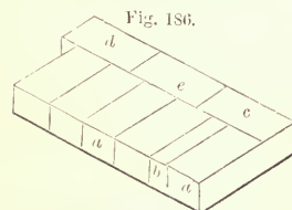
Fig. 186. PLAN OF SECOND COURSE OF 9-INCH WALL —SCALE, \frac{1}{2} INCH TO THE FOOT.
