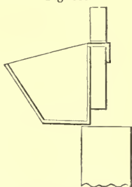
SECTION OF LATCOCK'S MANGER FOR CATTLE- BOXES—SCALE, \frac{1}{2} INCH TO THE FOOT.
