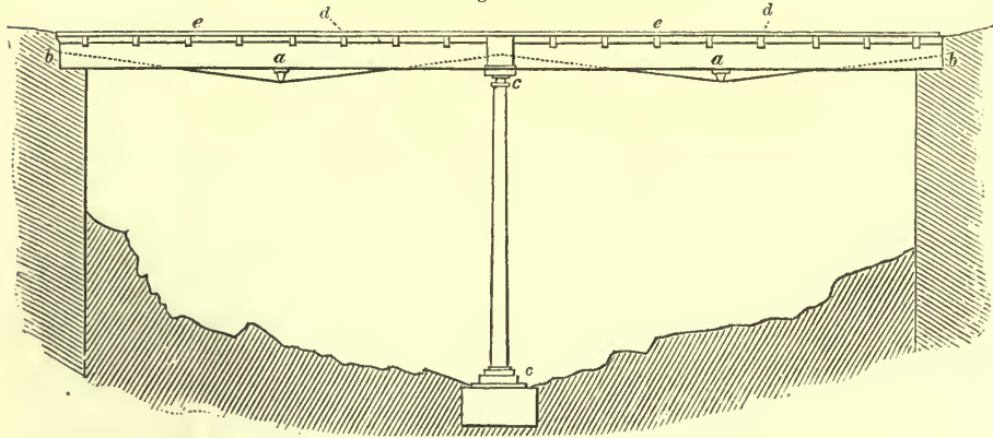
TRUSSED-GIRDER BRIDGE FOR A SPAN OF 32 FEET—SCALE, \frac{1}{2} INCH TO THE FOOT.
