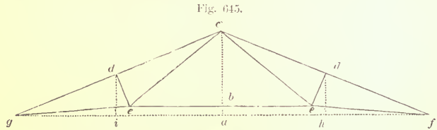
SKELTON OF IRON TRUSS FOR SPAN OF 25 FEET.—SCALE IN FIG. 657.
