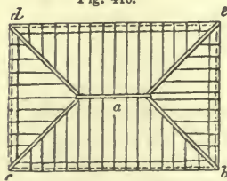
ROOF WITH HIP-RAFTER—SCALE, \frac{1}{8} INCH TO THE FOOT.
