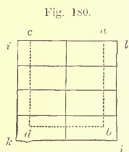
Fig. 180. PLAN OF THIRD COURSE OF FOOTINGS.—SCALE, \frac{1}{2} INCH TO THE FOOT.
