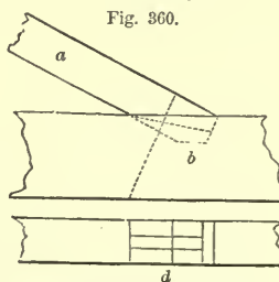
JOINING OF INCLINED BEAM WITH A HORIZONTAL BEAM—SCALE, \frac{1}{2} INCH TO THE FOOT.
