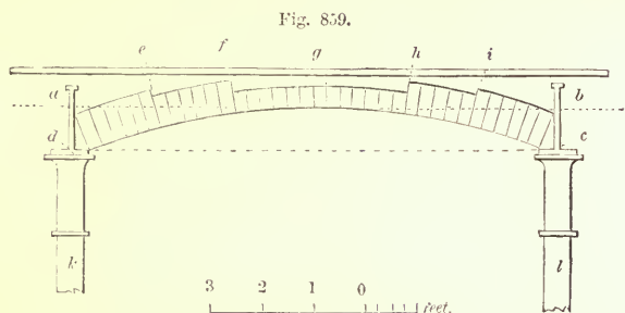
CAST-IRON GIRDERS, PILLARS, AND BRICK ARCHES, FOR FIREPROOF FLOORING
