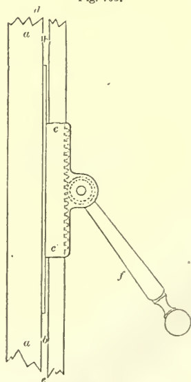
FASTENING FOR FRENCH OR CASEMENT WINDOWS—SIDE VIEW.
