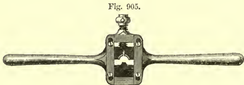
IBBOTSON'S SCREW-STOCK
