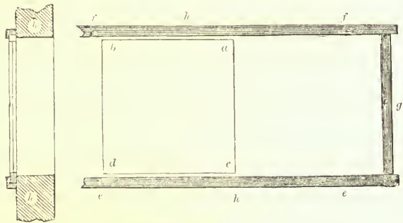
SECTION AND PLAN OF FRAME OF SLIDING WINDOW.
