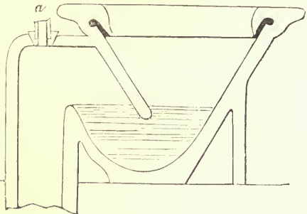
EARLY WATER-CLOSET PAN WITH TRAP
