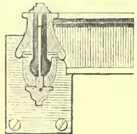
COLLINGE'S PATENT SPHERICAL HINGE.
