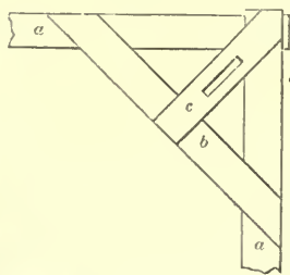
DRAGON-PIECE AND DIAGONAL TIE TO SUPPORT HIP-RAFTER.
