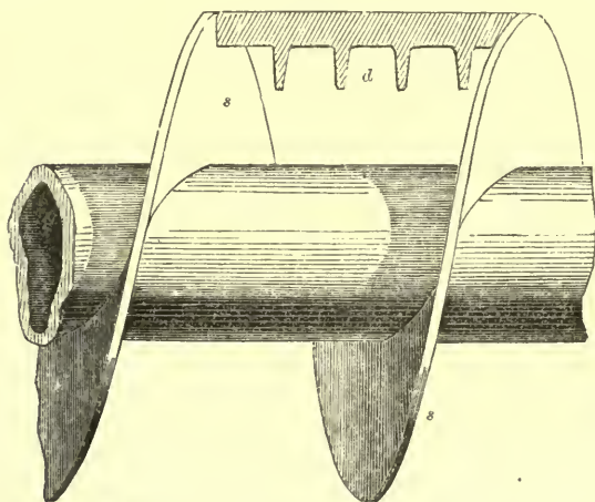
RAKE BETWEEN THE THREADS OF ARCHIMEDEAN SCREW CONVEYOR.
