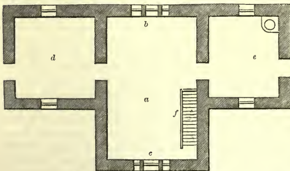
PLAN OF ISOLATED DAIRY—SCALE, \frac{1}{8} INCH TO THE FOOT.
