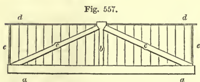
KING-POST TRUSS FOR BRIDGE—SCALE, \frac{1}{2} INCH TO THE FOOT.
