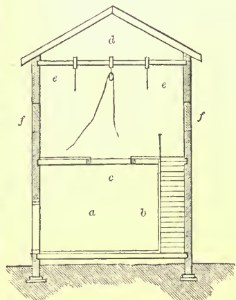
SECTION OF DETACHED SLAUGHTER-HOUSE— SCALE IN FIG. 946.
