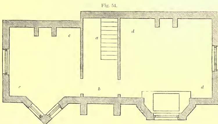
CELLAR-PLAN OF A SECOND-CLASS FARMHOUSE — SCALE IN FIG. 53.
