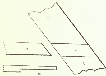
JOINT OF COLLAR BEAM WITH RAFTER—SCALE, \frac{1}{2} INCH TO THE FOOT.
