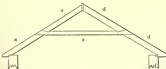
COLLAR-ROOF.
