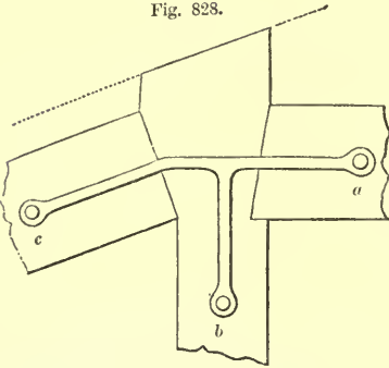
IRON STRAP FOR STRAINING-BEAM, QUEEN-POST, AND STRUT—SCALE, \frac{3}{4} INCH TO THE FOOT.
