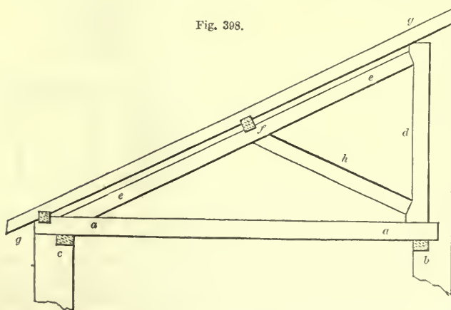
LEAN-TO ROOF, 20-FOOT SPAN—SCALE, ¼ INCH TO THE FOOT.
