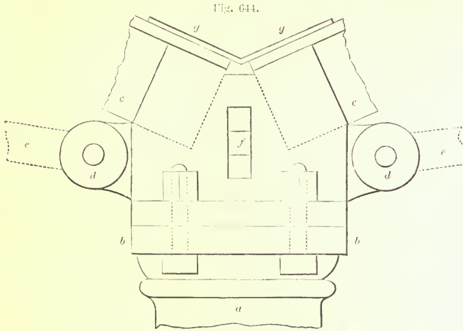
RAFTER-SHEATH FOR ROOF IN FIG. 643—SCALE IN FIG. 657.
