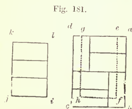
Fig. 181. PLAN OF FOURTH COURSE OF 14-INCH WALL.—SCALE, \frac{1}{2} INCH TO THE FOOT.
