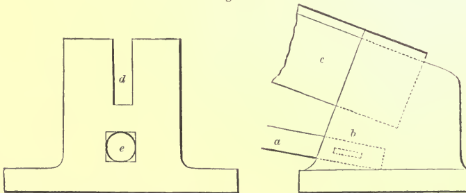
SIDE AND END ELEVATION OF RAFTER-SHOE.—SCALE IN FIG. 637.
