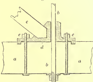
SHOE FOR QUEEN-BOLT AND STRUT—SCALE, \frac{1}{2} INCH TO THE FOOT.
