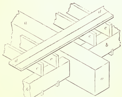
DOUBLE-FRAMED FLOORING—SCALE, \frac{1}{4} INCH TO THE FOOT.
