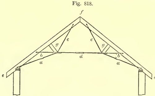
ROOF TRUSS OF OCTAGONAL SHED—SCALE, \frac{1}{8} INCH TO THE FOOT.
