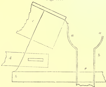
GUTTER FOR DOUBLE-SPAN ROOF—SCALE IN FIG. 657.
