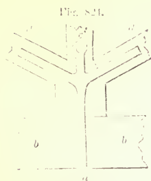
IRON STRAP FOR HEAD OF KING-POST, BRACES, AND COLLAR BEAM—SCALE, \frac{1}{4} INCH TO THE FOOT.
