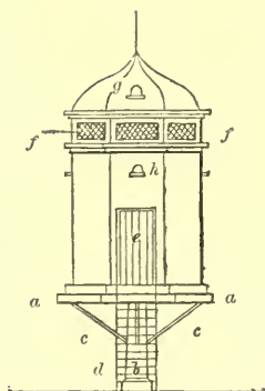
ELEVATION OF DETACHED PIGEON-HOUSE—SCALE, \frac{1}{16} INCH TO THE FOOT.
