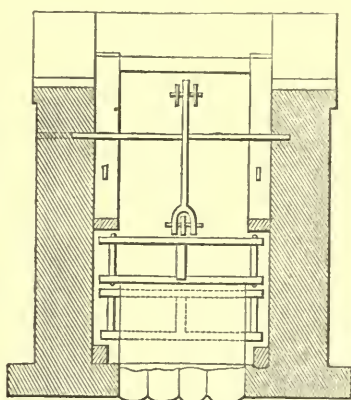
TRANSVERSE SECTION OF SELF-ACTING SLUICE.
