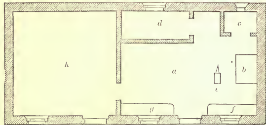
GROUND-PLAN OF SMITHY—SCALE, \frac{1}{16} INCH TO THE FOOT.
