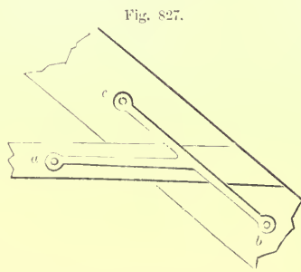
IRON STRAP FOR COLLAR AND RAFTER—SCALE, \frac{1}{4} INCH TO THE FOOT.
