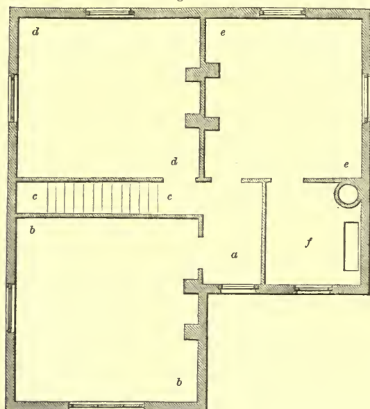
GROUND-PLAN OF A THIRD-CLASS FARMHOUSE—SCALE, \frac{3}{16} OF AN INCH TO THE FOOT.
