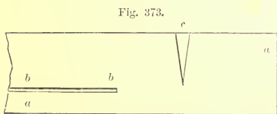
END OF BOW-AND-STRING RAFTER—SCALE, \frac{3}{4} INCH TO THE FOOT.
