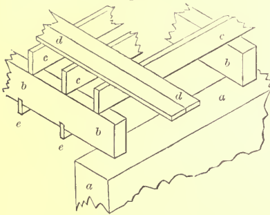
DOUBLE FLOORING—SCALE, \frac{1}{4} INCH TO THE FOOT.
