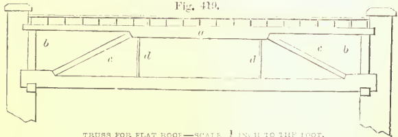
TRUSS FOR FLAT ROOF—SCALE, \frac{1}{4} INCH TO THE FOOT.
