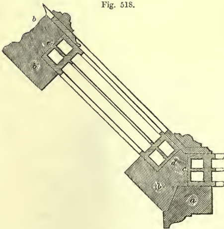
PLAN OF BAY WINDOW, CHAMBER FLOOR, IN FIG. 69—SCALE IN FIG. 516.
