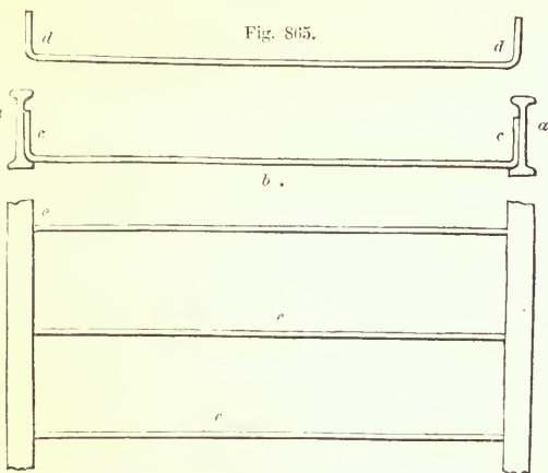
PLAN AND ELEVATION OF FIREPROOF FLOORING—SCALE, 3 INCH TO THE FOOT.
