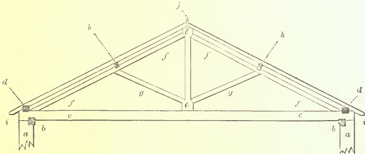
KING-POST TRUSS FOR 25-FOOT SPAN—SCALE, \frac{1}{8} INCH TO THE FOOT.
