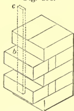
11-INCH HOLLOW WALL—SCALE, \frac{1}{2} INCH TO THE FOOT.
