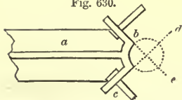
JUNCTION OF FOUR GIRDERS ON CAP OF COLUMN—SCALE, \frac{1}{2} INCH TO THE FOOT.
