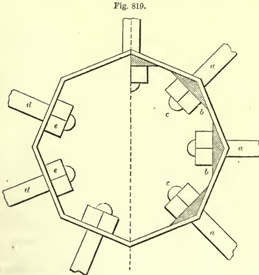
PLAN OF CENTRAL RING d , FIG. 818—SCALE, \frac{1}{8} INCH TO THE FOOT.
