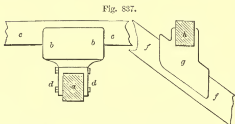
SHOE FOR "PURLINS"—SCALE \frac{1}{2} INCH TO THE FOOT.
