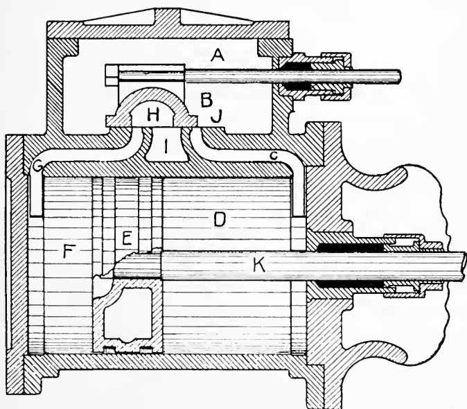
FIG. 243—CYLINDER AND VALVE OF STEAM ENGINE
