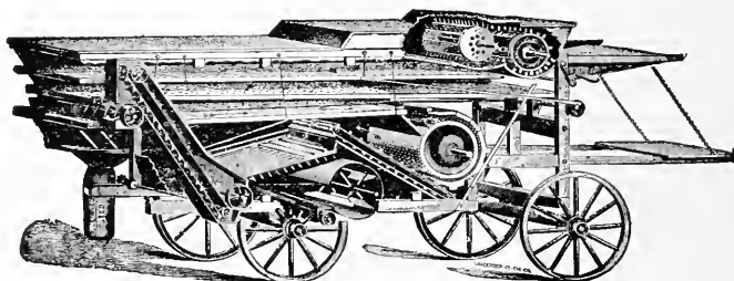
FIG. 166—SECTION OF A CLOVER HULLER
