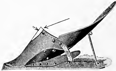
FIG. 49—THE BEARING SURFACE REQUIRED AT THE WING OF THE SHARE
