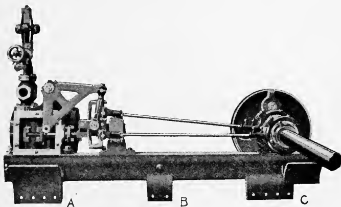
FIG. 330—ILLUSTRATING METHOD OF MOUNTING ENGINE ON BOILER
