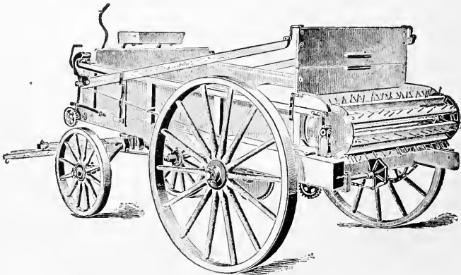
FIG. 151—A MANURE SPREADER WITH AN END BOARD TO BE PLACED IN FRONT OF THE BEATER
