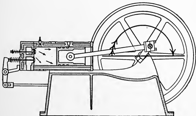
FIG. 281—SUCTION STROKE OF FOUR-CYCLE ENGINE
