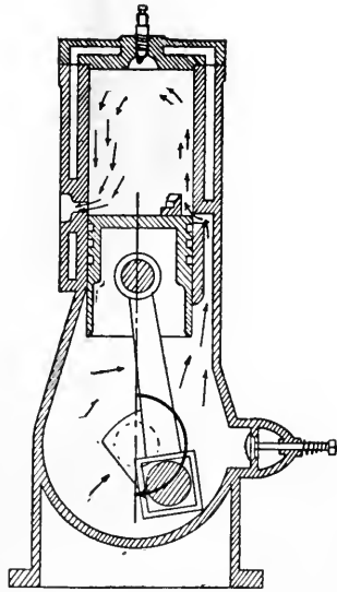
FIG. 288—EXPANSION, EXHAUST AND INLET STROKE OF TWO-CYCLE ENGINE
