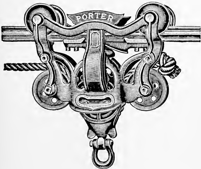
FIG. 140—A TWO-WAY FORK HAY CARRIER. TO WORK IN THE OPPOSITE DIRECTION, THE ROPE IS SIMPLY PULLED THROUGH UNTIL THE KNOT ON THE OPPOSITE END IS STOPPED BY THE CARRIER
