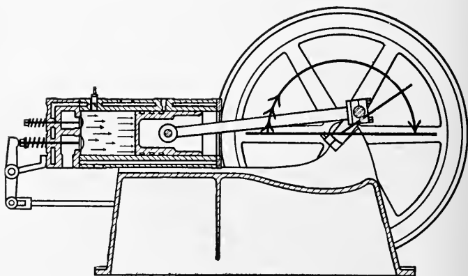
FIG. 283—EXPANSION AND RELEASE STROKE OF FOUR-CYCLE ENGINE
