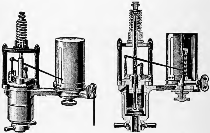
FIG. 14—THE STEAM OR GAS ENGINE INDICATOR. AN INSTRUMENT USED TO OBTAIN A RECORD OF THE PRESSURE IN THE ENGINE CYLINDER AT VARIOUS POINTS OF THE STROKE
