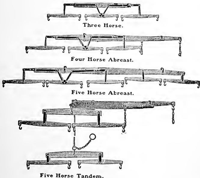
FIG. 3—GOOD TYPES OF EVENERS WHICH WILL DIVIDE EQUALLY THE DRAFT
