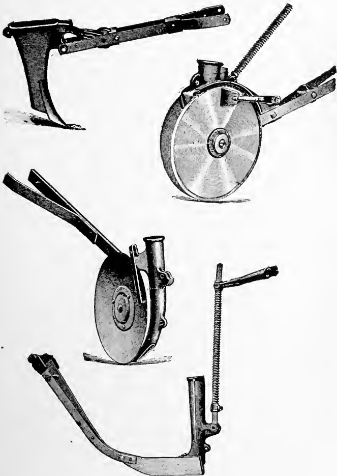
FIG. 85—THE HOE, DOUBLE-DISK, SINGLE-DISK, AND SHOE FURROW OPENERS USED ON DRILLS. THESE ARE OFTEN MADE INTERCHANGEABLE
