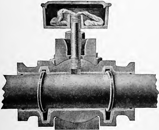
FIG. 26—A SELF-OILING AND SELF-ALIGNING BEARING. OFTEN THE OIL RESERVOIR BELOW THE RINGS IS ENLARGED AND THE WICK DISPENSED WITH
