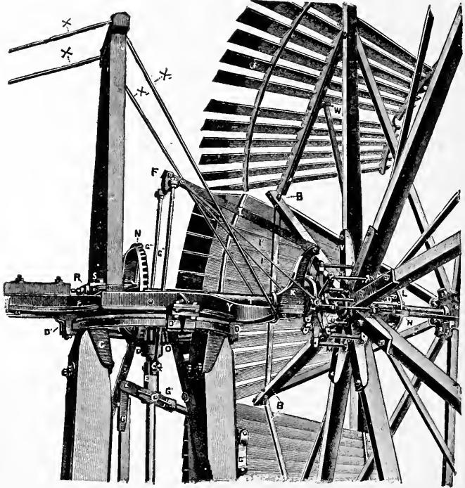
FIG. 206—SECTIONAL WHEEL WITH CENTRIFUGAL GOVERNOR AND INDEPENDENT RUDDER
