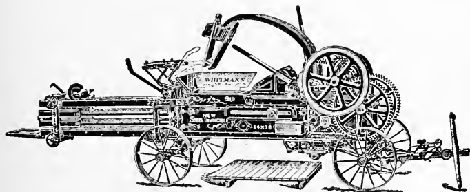
FIG. 144—A HAY PRESS FOR ENGINE POWER AND EQUIPPED WITH A CONDENSER TO THRUST THE HAY INTO THE HOPPER
