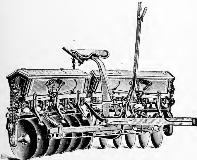
FIG. 82—A COMBINED DISK HARROW AND SEEDER. THIS MACHINE MAY ALSO BE SET TO DRILL FROM SEED SPOUTS AT THE REAR
