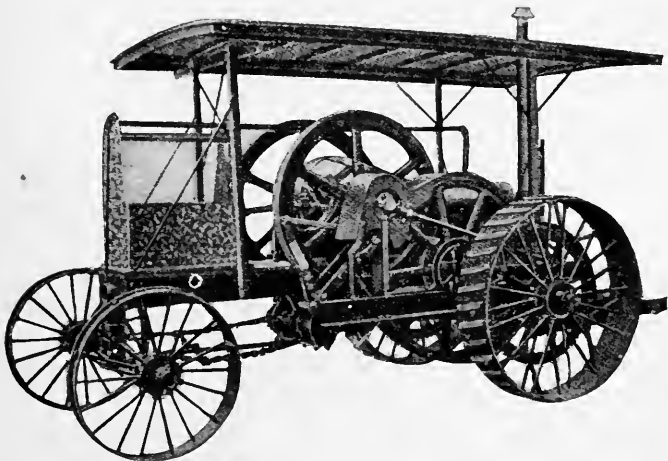
FIG. 337—GASOLINE TRACTION ENGINE WITH FRICTION GEARING
