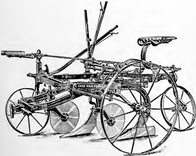
FIG. 39—THE MODERN GANG PLOW
