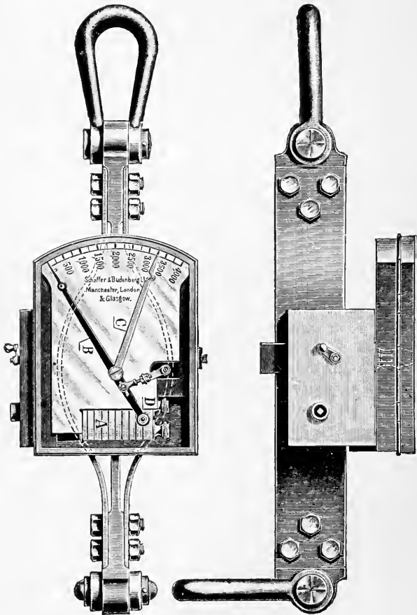
FIG. 12—GIDDINGS RECORDING DYNAMOMETER, WHICH HAS THE REEL DRIVEN BY CLOCK-WORK
