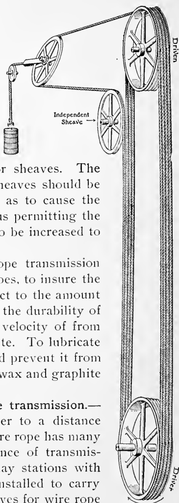
FIG. 20—TRANSMISSION OF POWER BY ROPES
