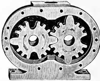
FIG. 194—SECTION OF A ROTARY PUMP SHOWING PISTONS
