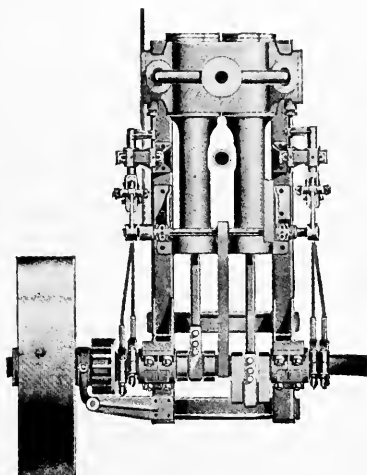
FIG. 276—DOUBLE-CYLINDER ENGINE
