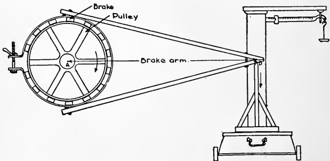
FIG. 7—PRONY BRAKE: ONE FORM OF ABSORPTION DYNAMOMETER
