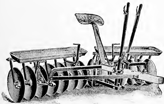
FIG. 55—A TWO-LEVER DISK HARROW. SCRAPERS OPERATED BY THE FEET
