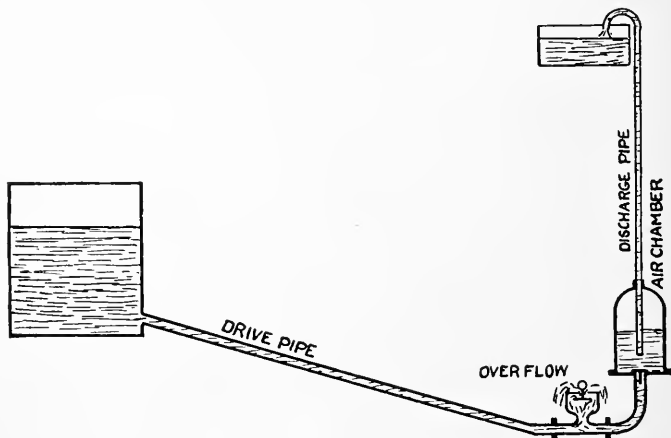
FIG. 196—HYDRAULIC RAM IN OUTLINE
