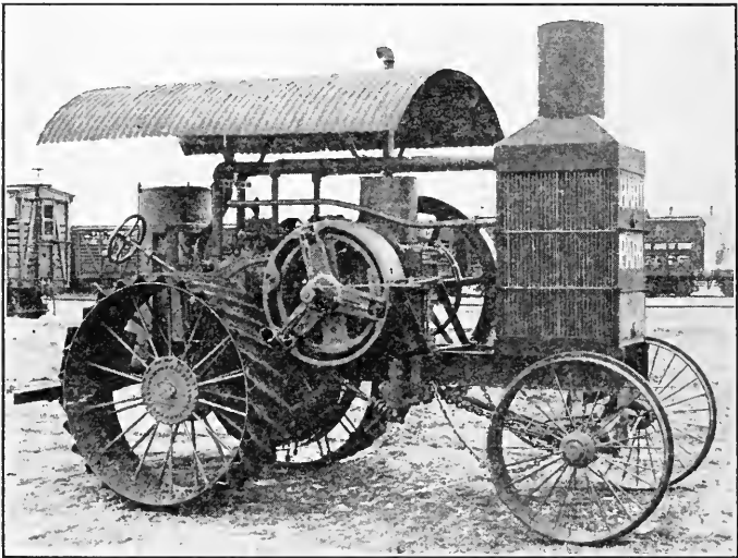
FIG. 338—TRACTION ENGINE WHICH REVERSES IN THE CLUTCH
