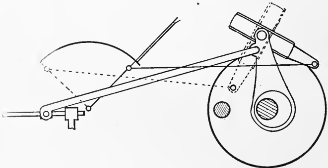
FIG. 262—PRINCIPLE OF WOOLF REVERSE GEAR
