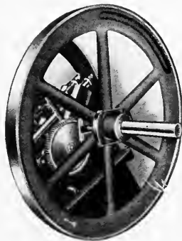
FIG. 299—FLYWHEEL GOVERNOR
