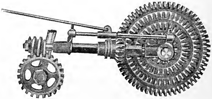
FIG. 153—THE WORM GEAR DRIVE TO THE APRON. ALSO FACE GEAR FOR VARYING THE FEED
