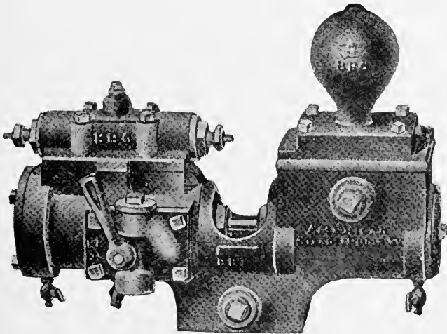
FIG. 227—INDEPENDENT DIRECT-ACTING PUMP
