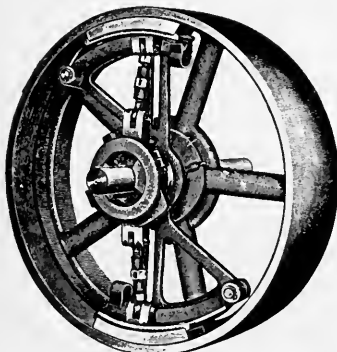
FIG. 333—CLUTCH WITH METAL BLOCKS
