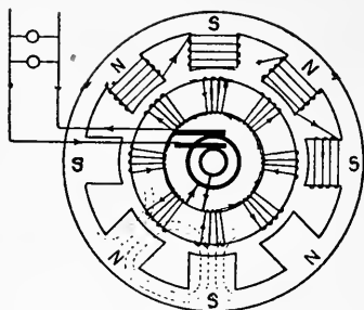
FIG. 359—SYSTEM OF WIRING FOR A MULTIPOLAR ALTERNATOR
