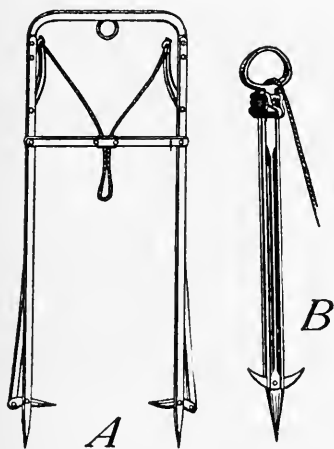
FIG. 137— A , DOUBLE-HARPOON HAY FORK. B , SINGLE-HARPOON HAY FORK
