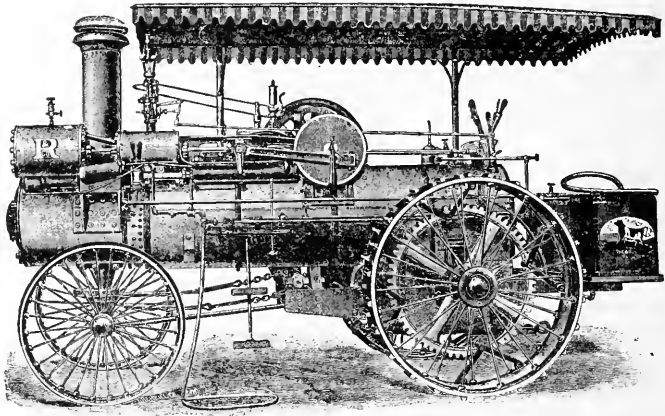
FIG. 317—SIDE-MOUNTED TRACTION ENGINE
