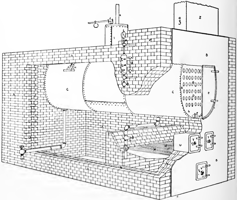
FIG. 215—EXTERNALLY FIRED BOILER
