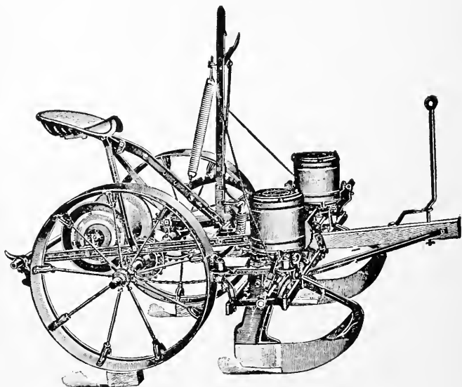
FIG. 89—A MODERN CORN PLANTER WITH LONG CURVED FURROW OPENERS, VERTICAL CHECK HEAD, AND OPEN WHEELS
