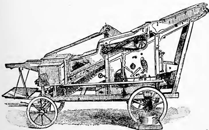
FIG. 155—THRESHING MACHINE OF 1867
