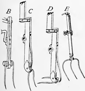
FIG. 129—TYPES OF TEDDER FORKS WITH COIL AND FLAT RELIEF SPRINGS. D SHOWS THE SPRING OF C SPRUNG
