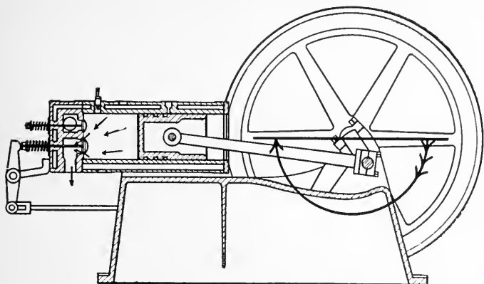
FIG. 284—EXHAUST STROKE OF FOUR-CYCLE ENGINE
