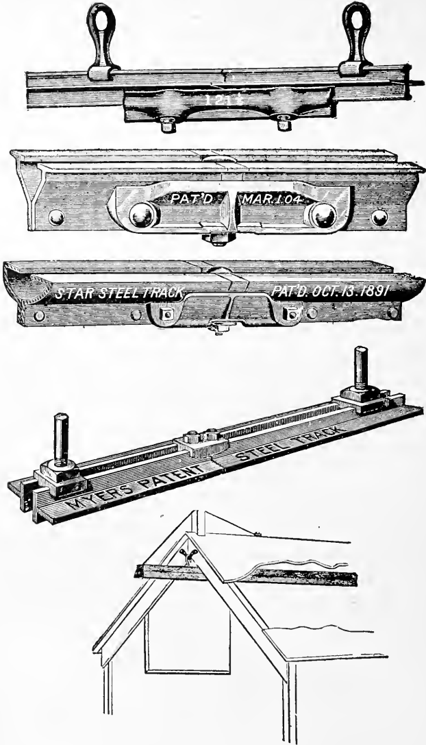
FIG. 136—TYPES OF STEEL AND WOOD HAY CARRIER TRACKS
