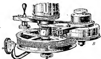
FIG. 267—REDUCING MOTION ATTACHED TO INDICATOR
