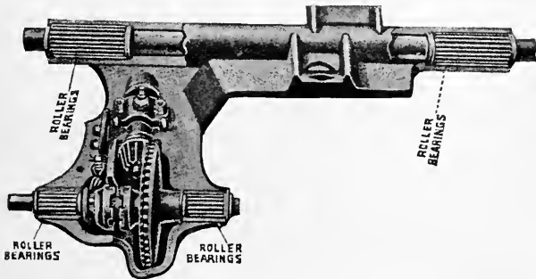
FIG. 25—ROLLER BEARINGS AS APPLIED TO A MOWER
