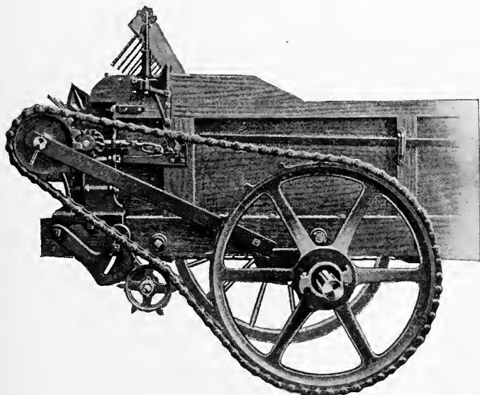
FIG. 149—A CHAIN AND GEAR DRIVE TO THE BEATER. THE BEATER IS PLACED IN GEAR BY MOVING BACK UNTIL GEARS MESH
