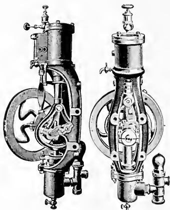
FIG. 228—INDEPENDENT PLUNGER PUMP
