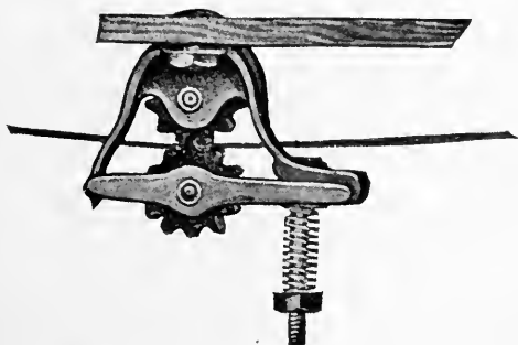
FIG. 112—A ROLLER TENSION FOR THE TWINE. A VERY SATISFACTORY DEVICE
