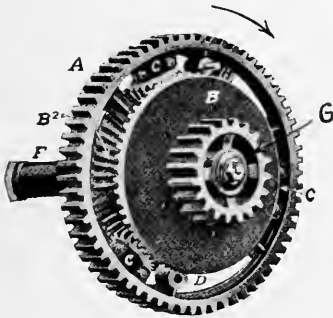
FIG. 335—COMPENSATING GEARS
