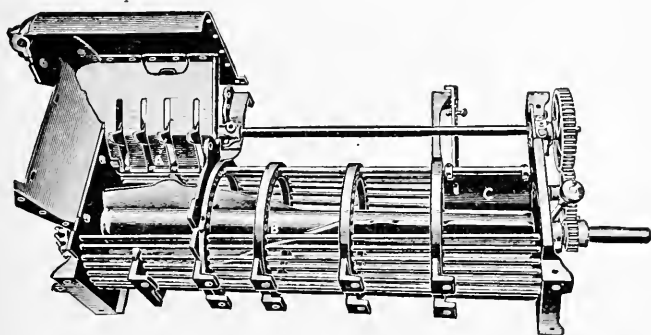
FIG. 173—SHELLING MECHANISM OF CYLINDER SHELLER
