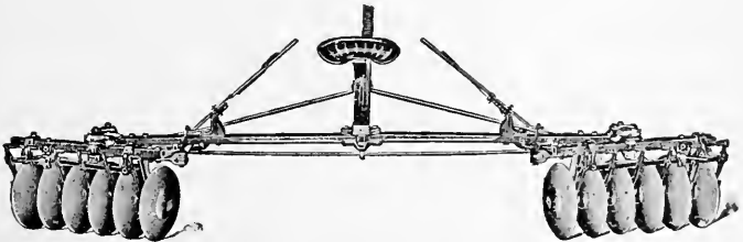
FIG. 58—AN ORCHARD DISK HARROW WITH WIDE FRAME TO WORK UNDER TREES. THE GANGS MAY BE SET TO THROW IN OR OUT
