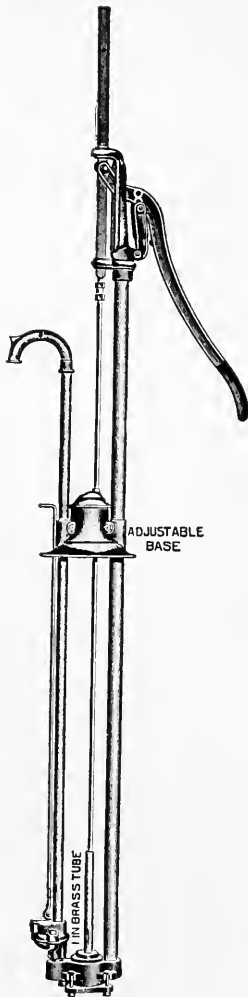
FIG. 191—A DOUBLE PIPE OR UNDERGROUND PUMP WITH STUFFING-BOX TUBE AND ADJUSTABLE BASE
