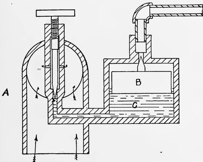
FIG. 305—PRINCIPLE OF THE FLOAT-FEED CARBURETOR
