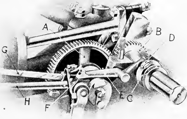
FIG. 297—MECHANISM FOR HIT-OR-MISS GOVERNOR
