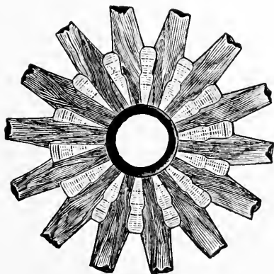
FIG. 181—A SECTION OF A WAGON HUB SHOWING THREE METHODS OF FORMING THE SPOKE SHOULDERS. THE ROUND SHOULDERS ARE SAID TO BE MUCH STRONGER AND MORE DURABLE
