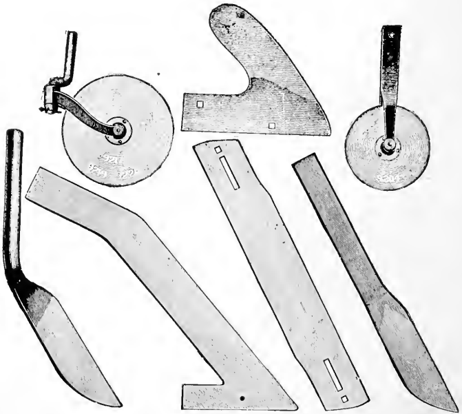
FIG. 37—ROLLING CASTER AND ROLLING STATIONARY COULTERS, FIN HANGING, KNEE, DOUBLE ENDER, AND KNIFE CUTTERS OR COULTERS
