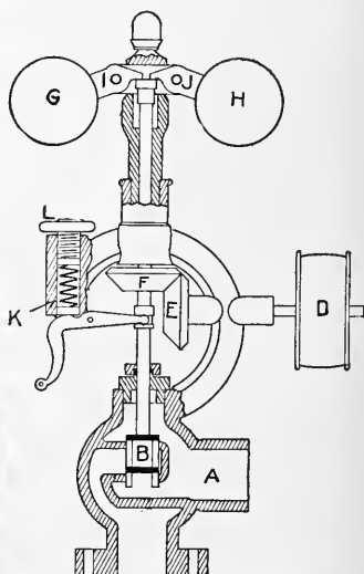
FIG. 272 —SECTIONAL VIEW OF THROTTLING GOVERNOR
