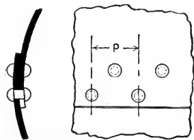
FIG. 239—DOUBLE-RIVETED LAP JOINT
