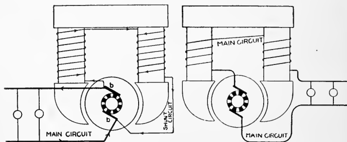
FIG. 363—SHUNT-WOUND DYNAMO FIG. 364—SERIES-WOUND DYNAMO
