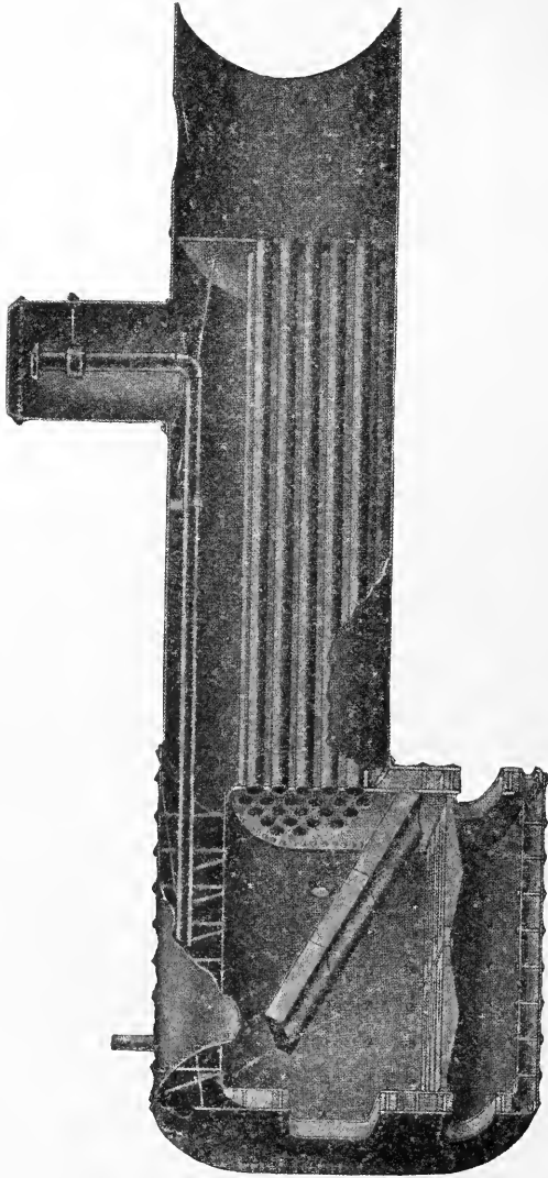
FIG. 216—LOCOMOTIVE TYPE OF INTERNALLY FIRED BOILER
