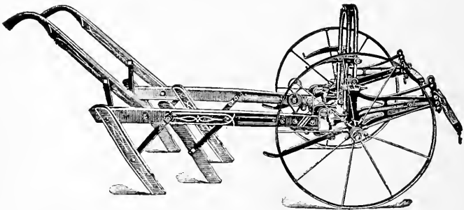
FIG. 65—A TONGUELESS FOUR-SHOVEL CULTIVATOR WITH WOODEN GANGS. THE SHOVELS ARE NOT IN PLACE
