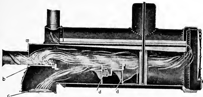
FIG. 223.—STRAW BURNER RETURN-FLUE BOILER
