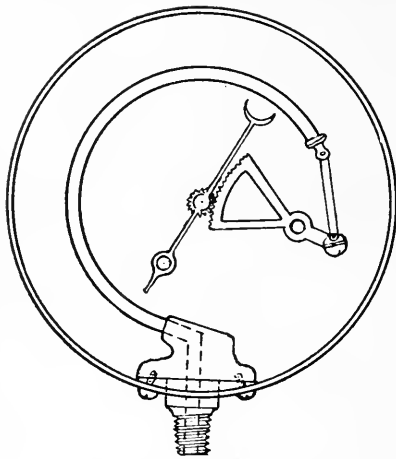
FIG. 233—STEAM GAUGE
