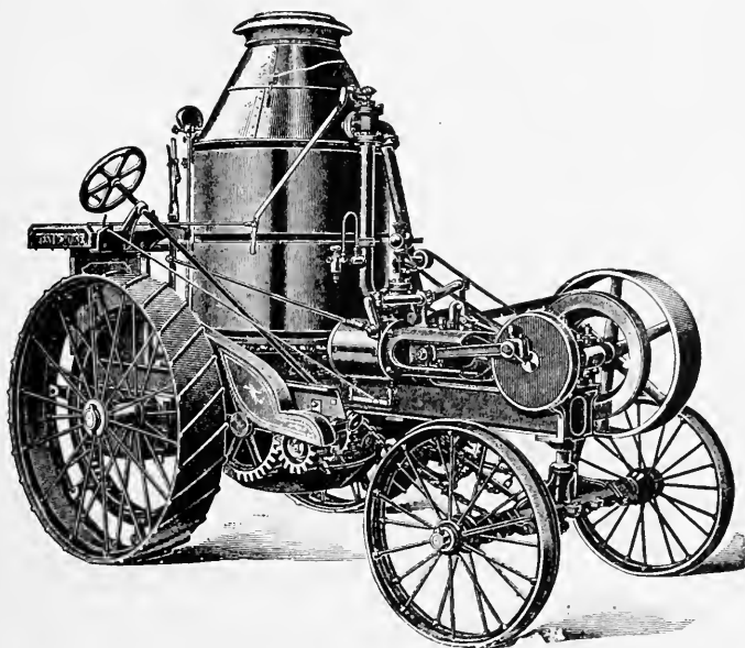
FIG. 327—FRAME-MOUNTED VERTICAL TRACTION ENGINE
