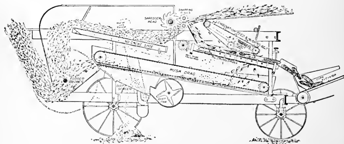
FIG. 170—SECTIONAL VIEW OF A HUSKER AND SHREDDER
