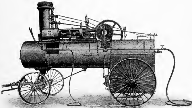
FIG. 316—SIDE-MOUNTED PORTABLE ENGINE
