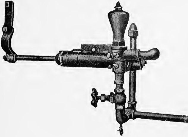
FIG. 226—CROSSHEAD PUMP
