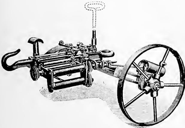
FIG. 11—A GERMAN RECORDING DYNAMOMETER WHICH HAS THE REEL DRIVEN BY CLOCK-WORK
