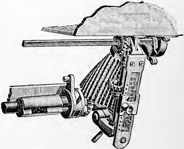
FIG. 80—A FEED-REGULATING DEVICE USED IN CONNECTION WITH A FORCE FEED SIMILAR TO THAT SHOWN IN FIG. 79
