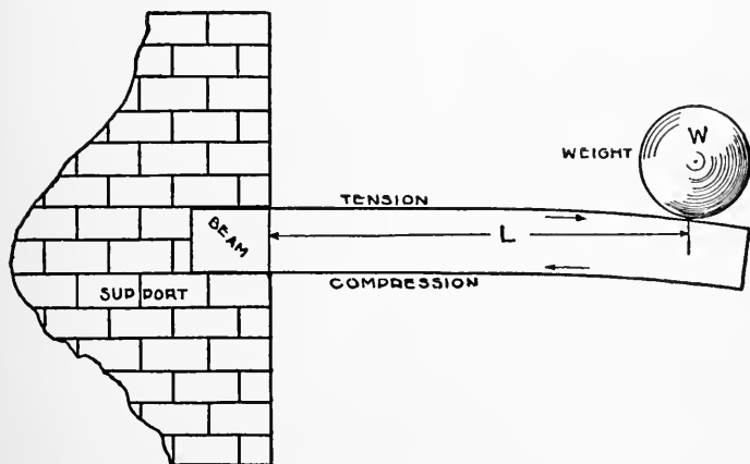
FIG. 28—A CANTILEVER BEAM
