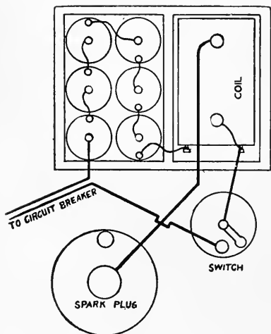
FIG. 308—WIRING SYSTEM FOR JUMP-SPARK IGNITION
