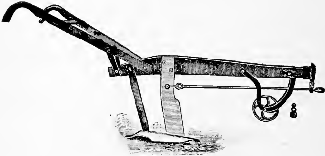
FIG. 45—A SUBSOIL PLOW FOR LOOSENING THE SOIL IN THE BOTTOM OF THE FURROW MADE BY THE COMMON PLOW
