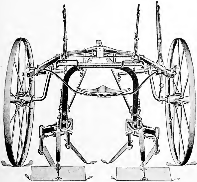
FIG. 68—A RIDING SURFACE CULTIVATOR
