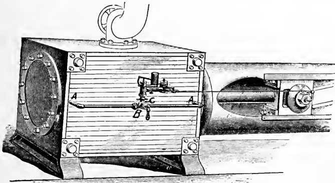
FIG. 266—ATTACHING AN INDICATOR TO AN ENGINE
