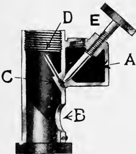
FIG. 302—PRINCIPLE OF THE CARBURETOR
