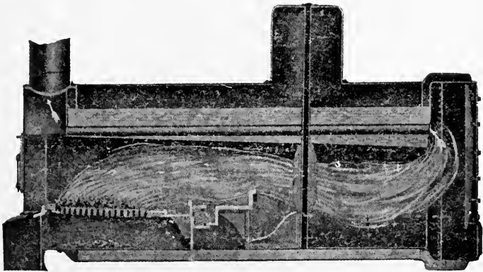
FIG. 217—RETURN-FLUE TYPE OF INTERNALLY FIRED BOILER
