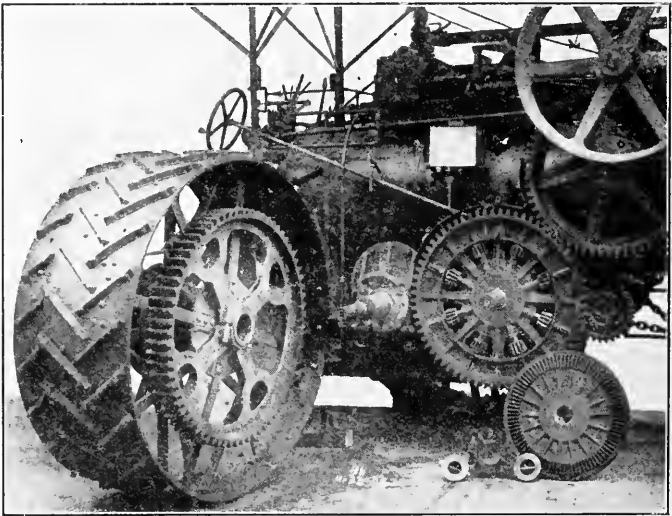
FIG. 334—GEARS CONNECTING ENGINE WITH TRACTION WHEELS
