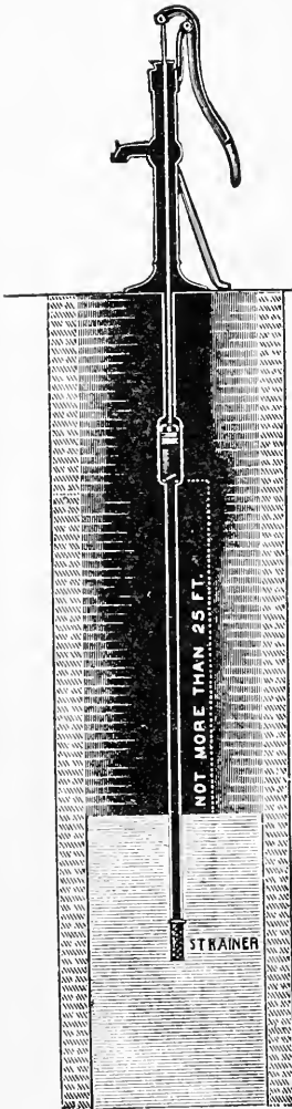
FIG. 189—A SUCTION PUMP IN A WELL
