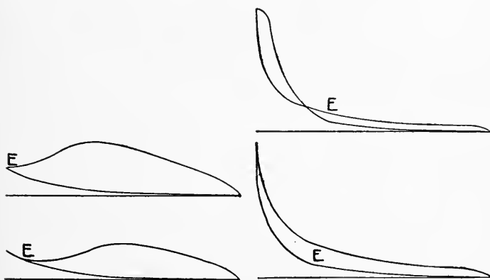
FIG. 313—TOO LATE IGNITION
