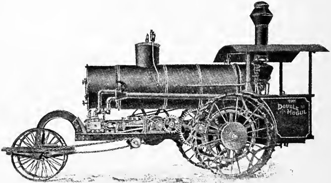
FIG. 328—FRAME-MOUNTED ENGINE OF THE LOCOMOTIVE TYPE
