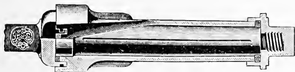
FIG. 185—A LONG-DISTANCE BUGGY AXLE. NOTE THE PROVISION MADE TO EXCLUDE DUST AND DIRT
