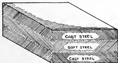
FIG. 27—DRAWING ILLUSTRATING THE CONSTRUCTION OF SOFT-CENTER STEEL
