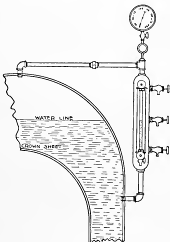
FIG. 232—WATER COLUMN, GAUGE GLASS, TRY COCKS AND STEAM GAUGE
