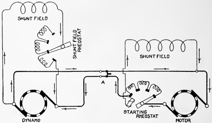
FIG. 368—WIRING SYSTEM FOR DYNAMO AND MOTOR
