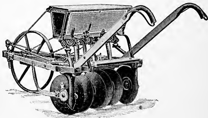
FIG. 87—A FIVE-DISK DRILL FOR DRILLING BETWEEN CORN ROWS. THE CENTER FURROW OPENER IS A DOUBLE DISK
