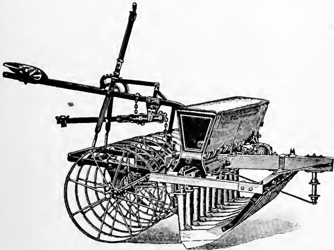
FIG. 83—A LOW-DOWN PRESS DRILL WITH SHOE FURROW OPENERS
