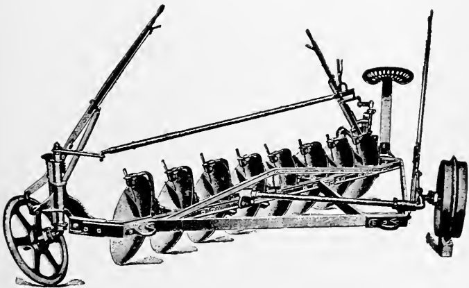
FIG. 47—AN ENGINE DISK GANG PLOW TURNING 8-, 10-, OR 12-INCH FURROWS
