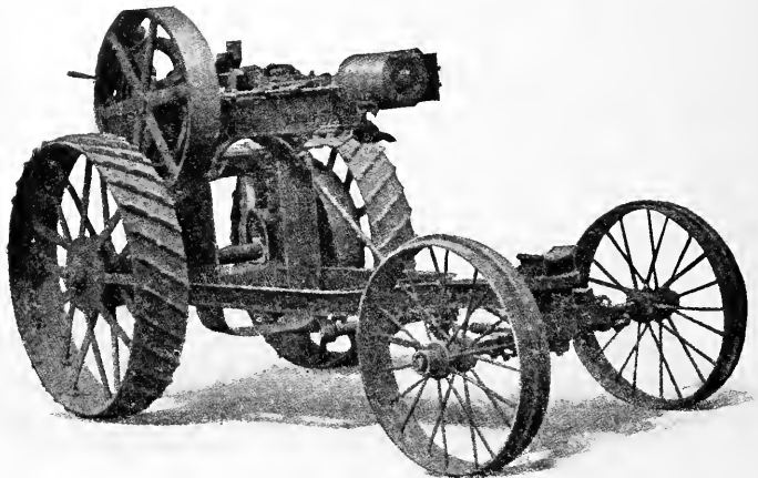
FIG. 326—FRAME-MOUNTED ENGINE
