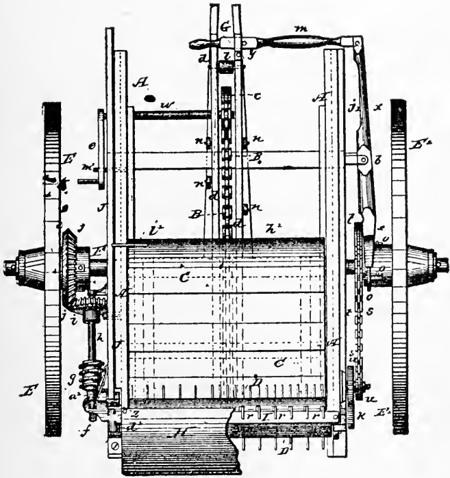
FIG. 145—THE J. S. KEMP MACHINE OF 1877. (FROM A PATENT OFFICE DRAWING)
