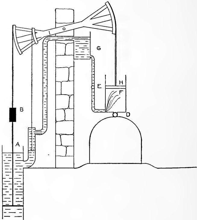
FIG. 242—NEWCOMEN'S ENGINE
