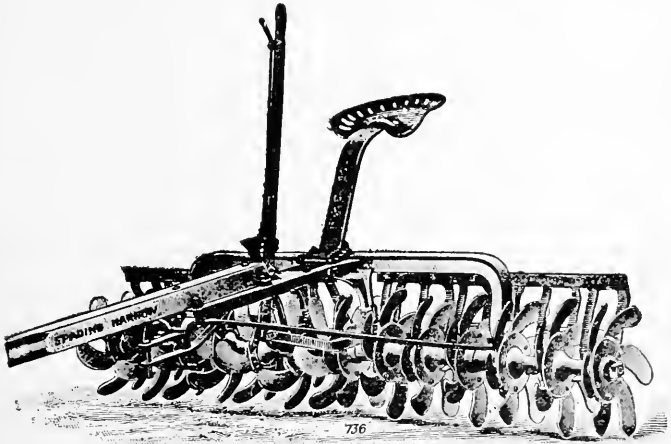
FIG. 57—A SPADING HARROW
