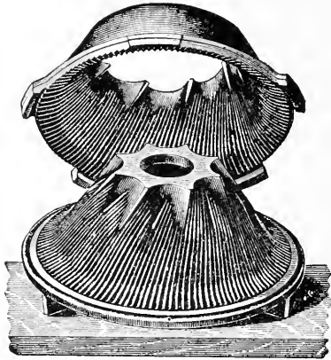
FIG. 176—BUHRS FOR A SWEEP MILL
