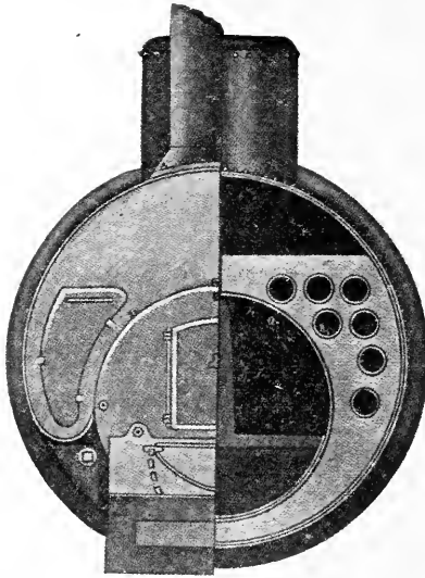
FIG. 221.—END VIEW OF RETURN-FLUE BOILER
