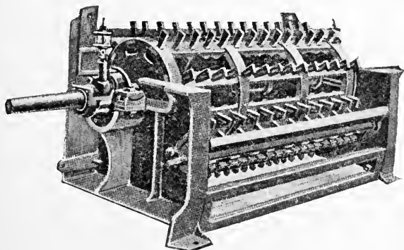
FIG. 157—THE CYLINDER AND CONCAVE
