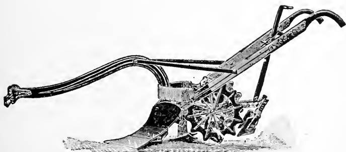
FIG. 99—A SINGLE-ROW WALKING LISTER WITH A CORN DRILL ATTACHED. DISKS ARE USED IN PLACE OF THE COVERING SHOVEL.
