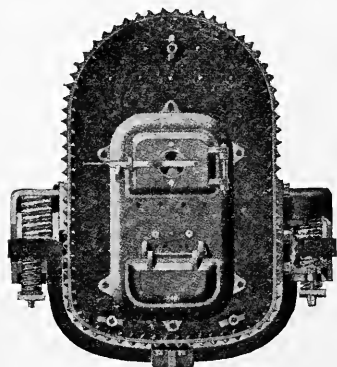
FIG. 320—SIDE-MOUNTED ENGINE WITH SPRINGS AND TRUSS BAR
