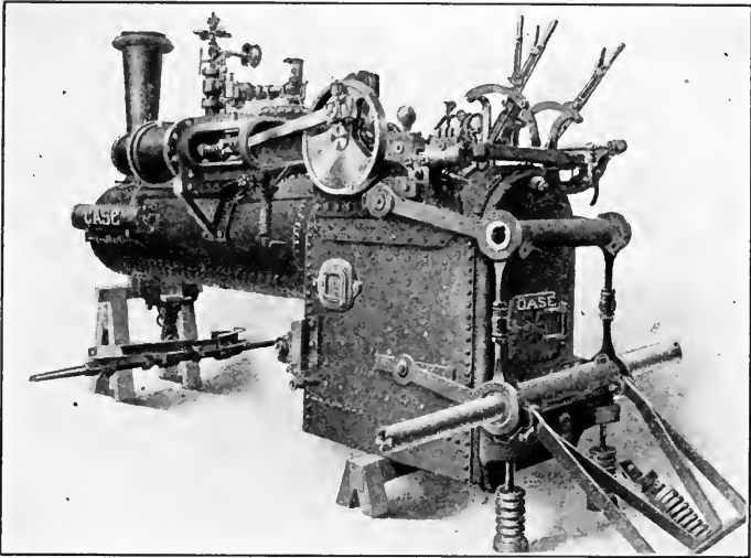
FIG. 323—REAR-MOUNTED ENGINE WITH RADIUS AND CROSS LINKS
