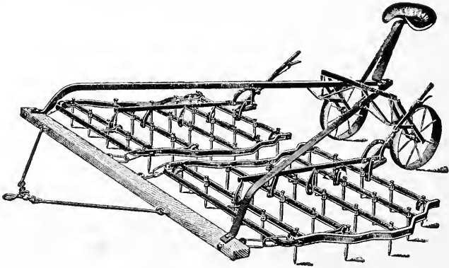
FIG. 54—A STEEL LEVER HARROW WITH A RIDING ATTACHMENT OR HARROW CART. THIS HARROW HAS THE TOOTH BARS MADE OF STEEL CHANNEL BARS WITH PROTECTED ENDS
