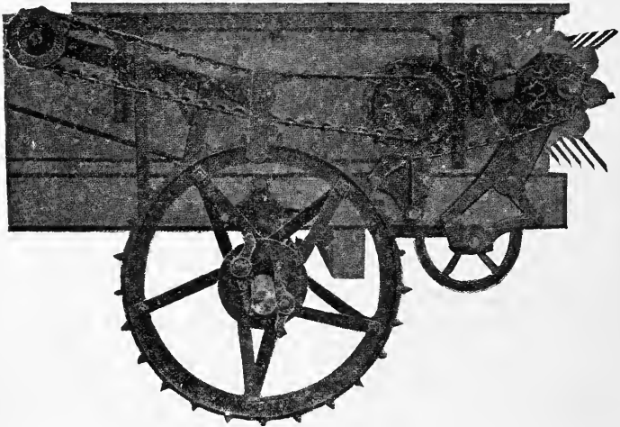
FIG. 148—A CHAIN DRIVE TO THE BEATER. NOTE THE METHOD OF REVERSING THE MOTION
