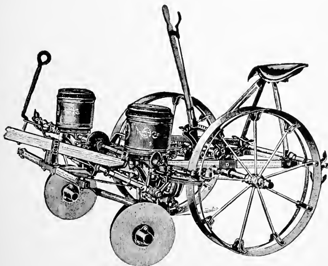
FIG. 96—A CORN PLANTER WITH DOUBLE-DISK FURROW OPENERS, OPEN WHEELS, AND HORIZONTAL CHECK HEADS
