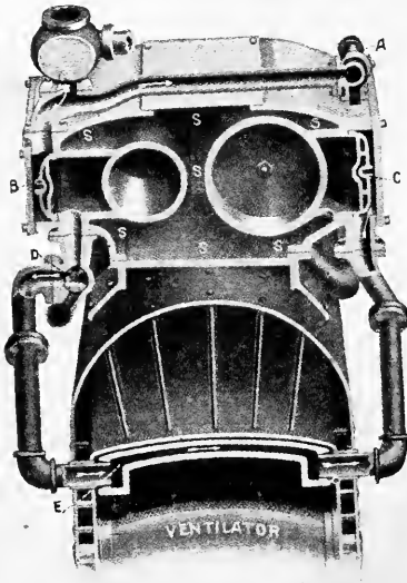
FIG. 278—CROSS-COMPOUND ENGINE
