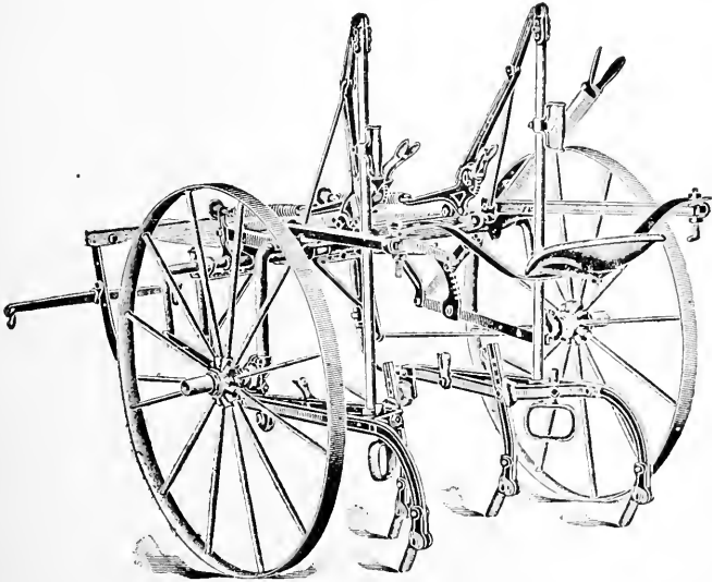
FIG. 66—A RIDING BALANCE-FRAME FOUR-SHOVEL CULTIVATOR WITH HAMMOCK SEAT AND STEEL GANGS
