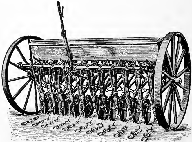
FIG. 86—A STANDARD SINGLE-DISK DRILL WITH COVERING CHAINS
