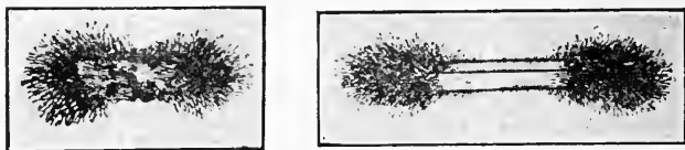
FIG. 339—NATURAL AND ARTIFICIAL MAGNETS ATTRACTING IRON FILINGS
