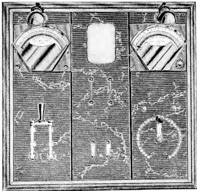
FIG. 369—COMMERCIAL SWITCHBOARD
