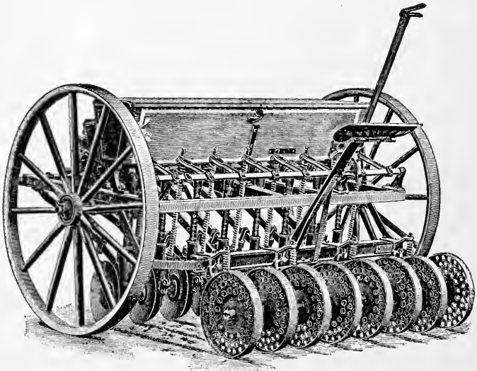
FIG. 84—A STANDARD SINGLE-DISK DRILL WITH A PRESS-WHEEL ATTACHMENT. THE STEEL RIBBON SEED TUBES ARE ALSO SHOWN
