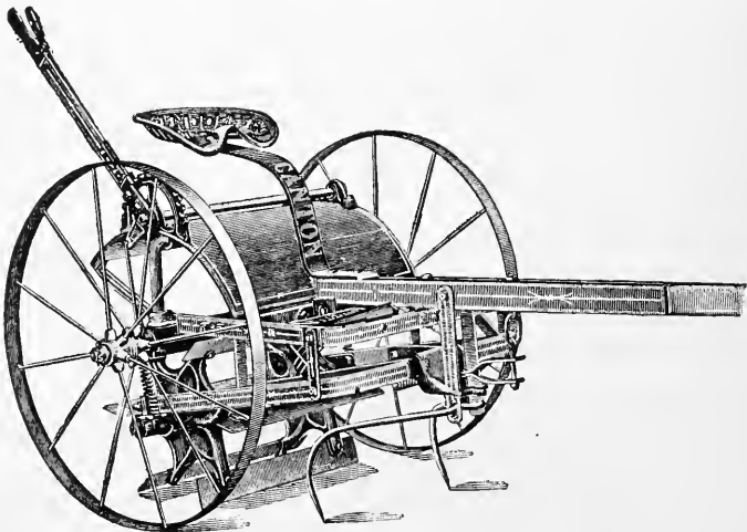
FIG. 73—A SINGLE-ROW STALK CUTTER
