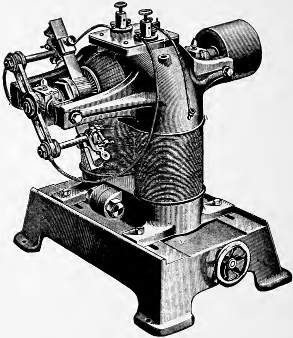
FIG. 365—BIPOLAR DIRECT-CURRENT DYNAMO
