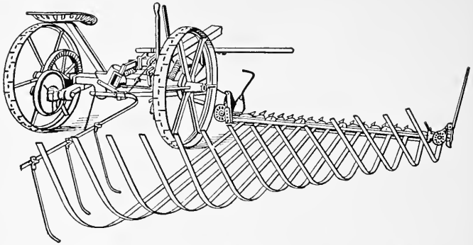
FIG. 123—A WINDROWING ATTACHMENT FOR A MOWER. IT MAY ALSO BE USED AS A BUNCHER
