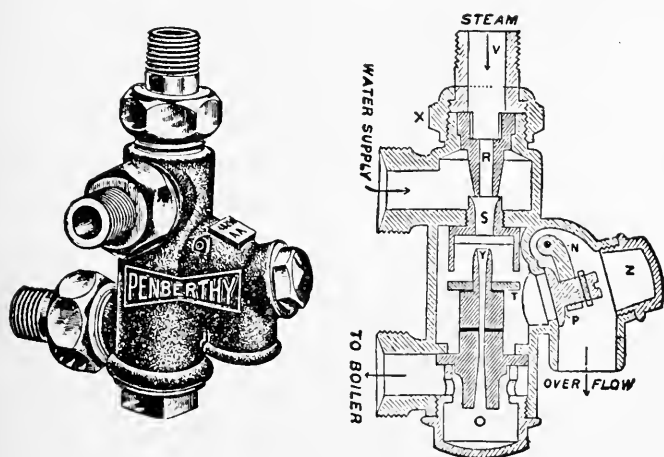
FIG. 230—COMMERCIAL INJECTOR
