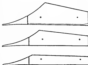
FIG. 36—THE FORM OF THE HIGH, MEDIUM, AND LOW LANDSIDES FOR WALKING PLOWS
