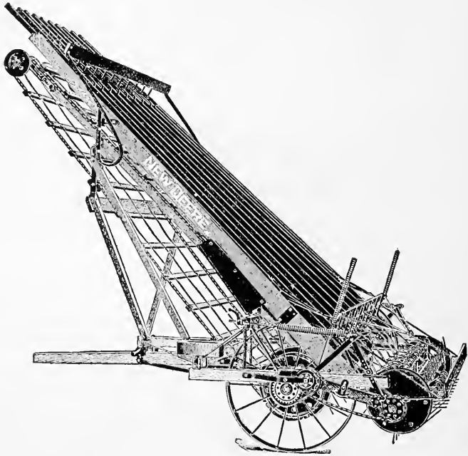
FIG. 131—AN ENDLESS APRON OR CARRIER HAY LOADER
