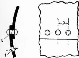
FIG. 238—SINGLE-RIVETED LAP JOINT
