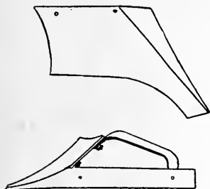
FIG. 35—STEEL PLOWSHARES. THE UPPER IS THE SLIP SHARE, AND THE LOWER THE BAR SHARE
