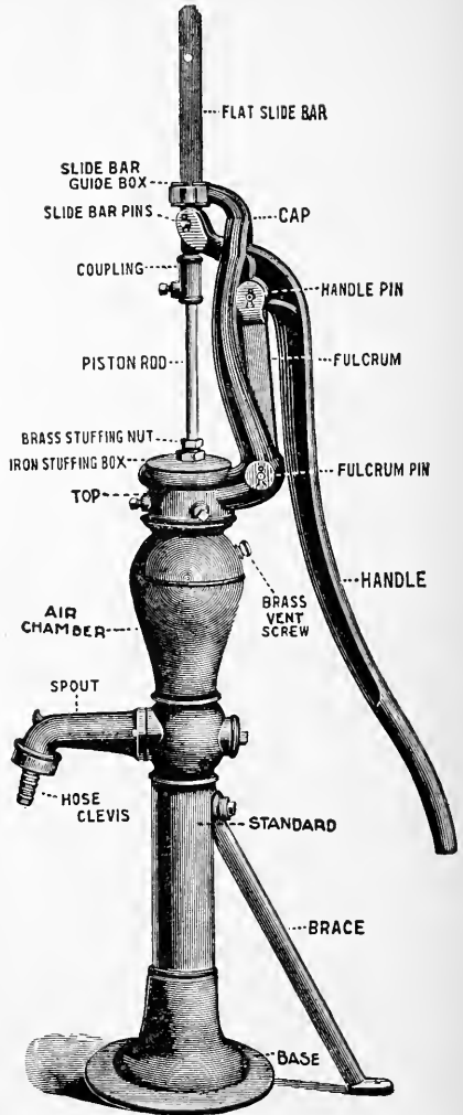
FIG. 190—A CAST-IRON PUMP STANDARD, WITH THE COMMON NAMES FOR ITS PARTS
