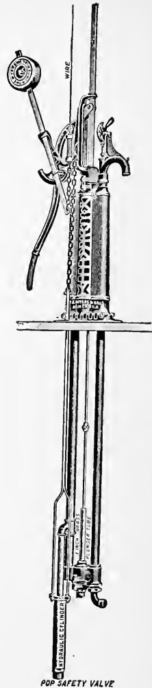
FIG. 192—AN UNDERGROUND PUMP WITH ORNAMENTAL BASE AND EQUIPPED WITH A WINDMILL REGULATOR
