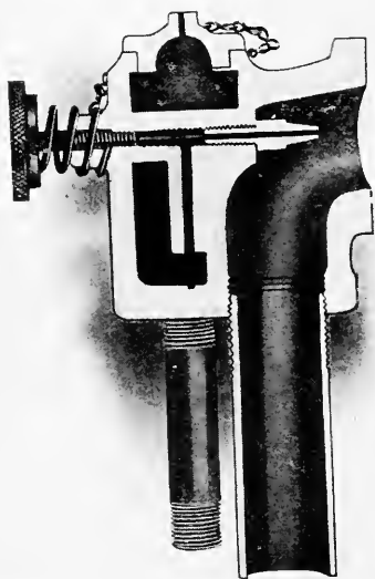
FIG. 303—CONSTANT-LEVEL CARBURETOR
