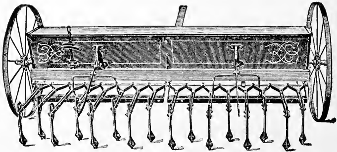
FIG. 77—AN AGITATOR-FEED BROADCAST SEEDER WITH CULTIVATOR COVERING SHOVELS. THIS IS A WIDE-TRACK MACHINE
