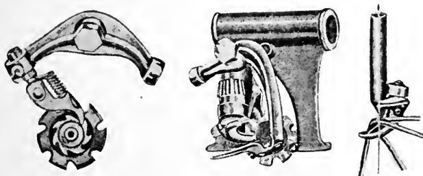
FIG. 113—A TWINE DISK. A KNOTTER COMPLETE—A KNOTTER HOOK
