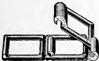
FIG. 18—MALLEABLE LINK BELTING OF ROTATING SHAFTS
