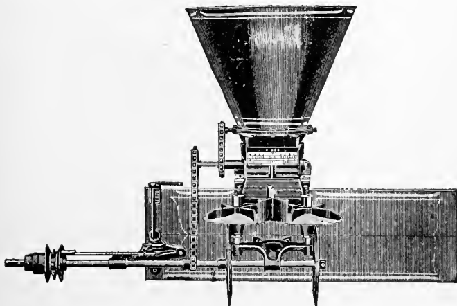
FIG. 76—AN END-GATE SEEDER WITH A FORCE FEED AND FRICTION GEARING. THIS MACHINE HAS TWO SEED DISTRIBUTERS
