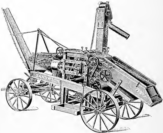
FIG. 174—A SIX-HOLE POWER SHELLER
