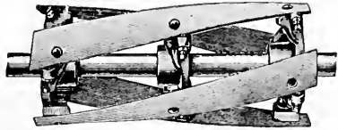
FIG. 169—A SPIRAL KNIFE CUTTER HEAD
