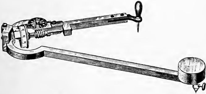
FIG. 13—THE PLANIMETER USED TO FIND THE AVERAGE DRAFT FROM DYNAMOMETER RECORDS. THERE ARE SEVERAL TYPES OF THIS INSTRUMENT
