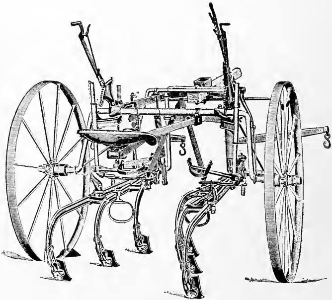
FIG. 67—A COMBINED WALKING AND RIDING SIX-SHOVEL CULTIVATOR WITH STRADDLE SEAT AND TREADLE GUIDE. THE HANDLES TO BE USED WHEN WALKING ARE NOT ATTACHED
