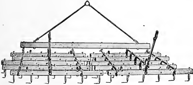
FIG. 50—A WOOD-BAR LEVER SMOOTHING HARROW. A CHEAPER HARROW IS MADE WITH FIXED TEETH AND A WOODEN FRAME
