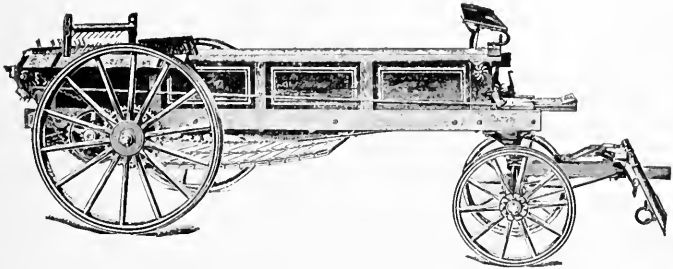
FIG. 146—A RETURN APRON SPREADER, SHOWING THE APRON UNDERNEATH, AND ALSO A GEAR AND CHAIN DRIVE TO BEATER
