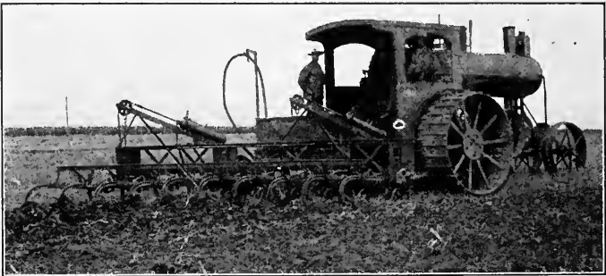
FIG. 329—LOCOMOTIVE TYPE OF TRACTION ENGINE WITH STEAM-OPERATED PLOW
