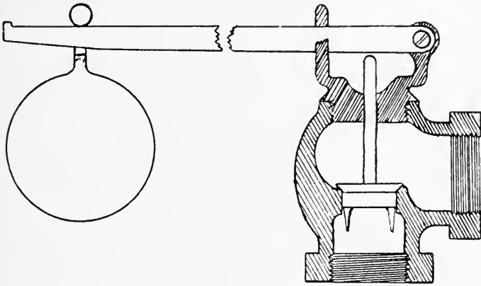
FIG. 235—BALL AND LEVER SAFETY VALVE
