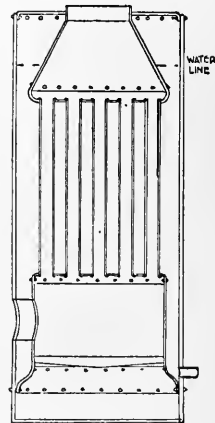
FIG. 213—VERTICAL BOILER WITH SUBMERGED FLUES
