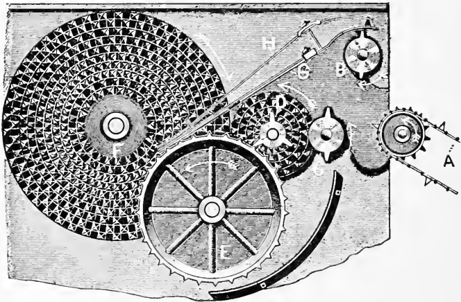
FIG. 172—SHELLING MECHANISM OF THE PICKER OR SPRING SHELLER. A, FEED CHAIN; B, C, BEATERS; D, F, PICKER WHEELS; E, BEVEL RUNNER; G, RAG IRON; H, SPRING
