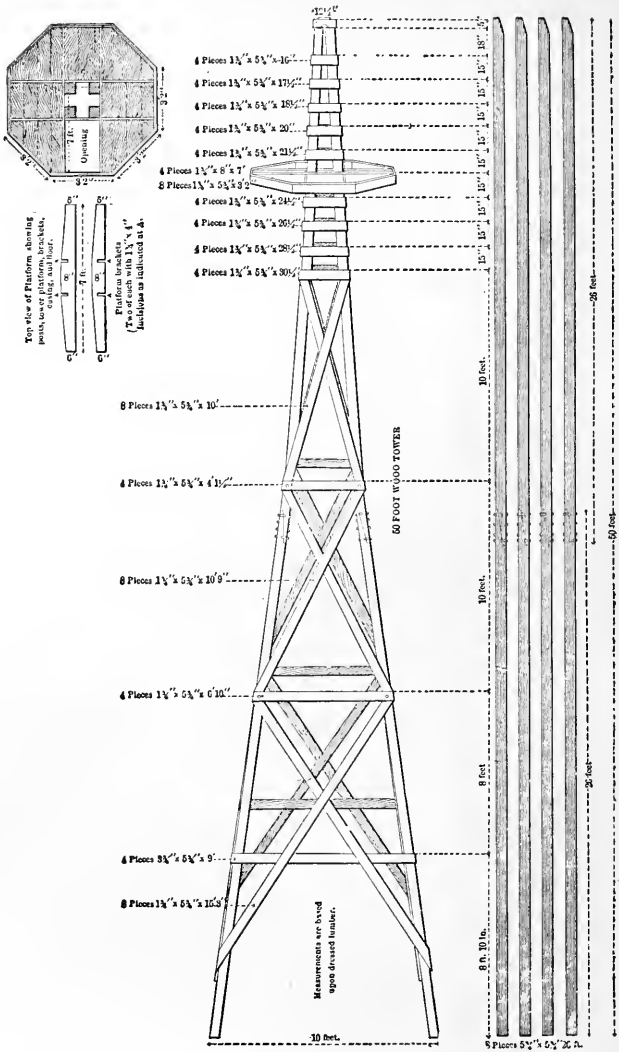
FIG. 210—DIMENSIONS FOR 50-FOOT TOWER
