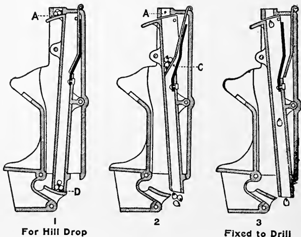
FIG. 93—A DOUBLE VALVE MECHANISM SHOWING HOW THE CORN IS RELEASED AT THE HEEL OF THE FURROW OPENER
