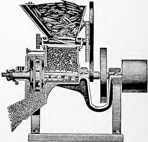
FIG. 178—A SECTIONAL VIEW OF A POWER MILL WITH DUPLEX BUHRS AND CRUSHING KNIVES
