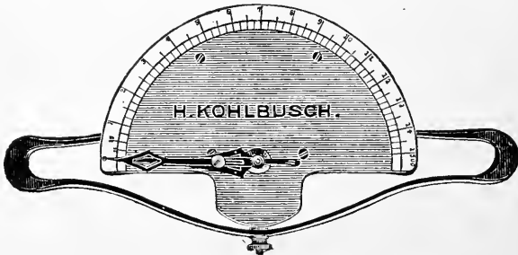
FIG. 9—DIRECT-READING DYNAMOMETER
