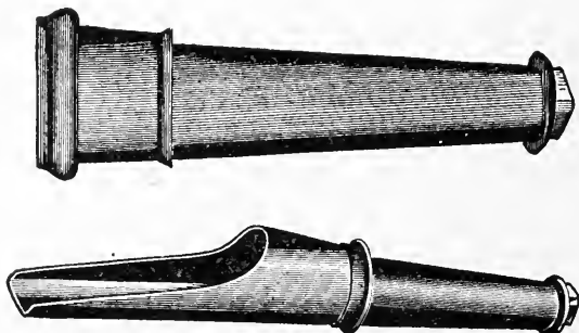
FIG. 182—THE UPPER IS THE CAST; THE LOWER, THE STEEL WAGON SKEIN
