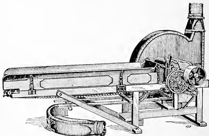
FIG. 167—AN ENSILAGE CUTTER WITH SELF-FEEDER AND PNEUMATIC ELEVATOR
