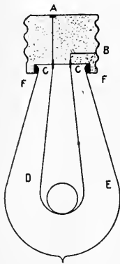
FIG. 370—INCANDESCENT LAMP
