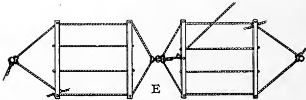
FIG. 139—A HAY SLING. THE SPRING CATCH BY WHICH THE SLING IS PARTED IS ABOVE E
