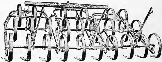
FIG. 53—A SPRING-TOOTH LEVER HARROW
