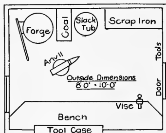
FIG. 375—ARRANGEMENT OF A SMALL SHOP
