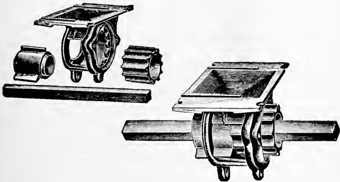
FIG. 78—A FORCE-FEED DEVICE. THE FEED IS VARIED BY EXPOSING MORE OR LESS OF THE FLUTED FEED SHELL
