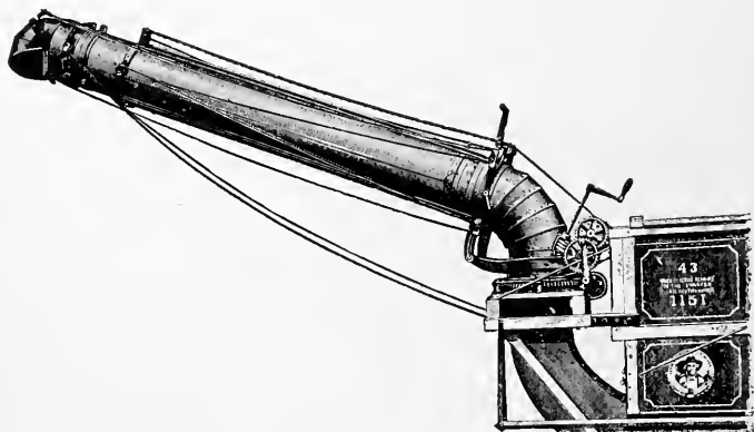
FIG. 163—A WIND STACKER. THE FAN DRUM IS NOT SHOWN
