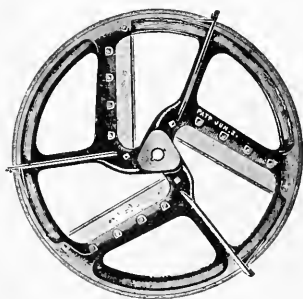
FIG. 168—A RADIAL KNIFE CUTTER HEAD
