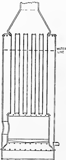
FIG. 212—VERTICAL BOILER
