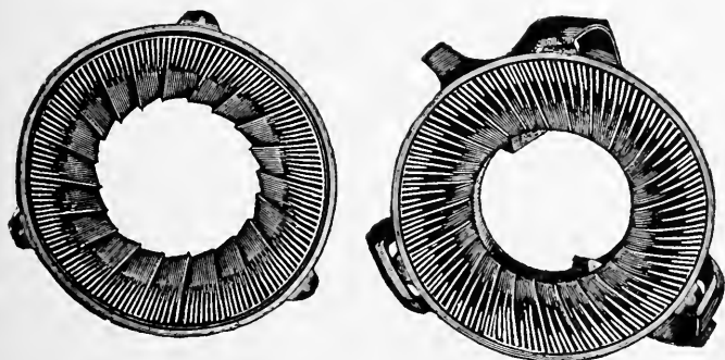
FIG. 175—CHILLED IRON BUHRS
