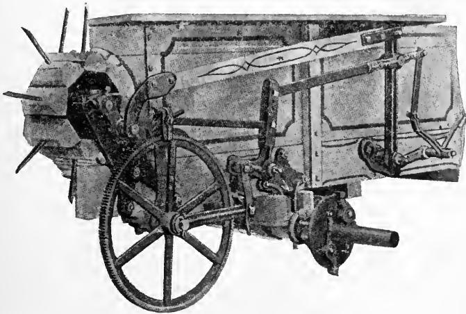
FIG. 152—A RATCHET DRIVE FOR THE APRON. NOTE METHOD OF VARYING THE FEED
