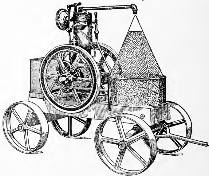
FIG. 311—CIRCULATING PUMP SYSTEM OF COOLING
