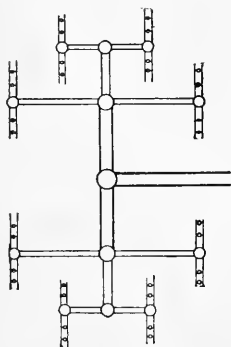
FIG. 371—PARALLEL CIRCUIT WIRING
