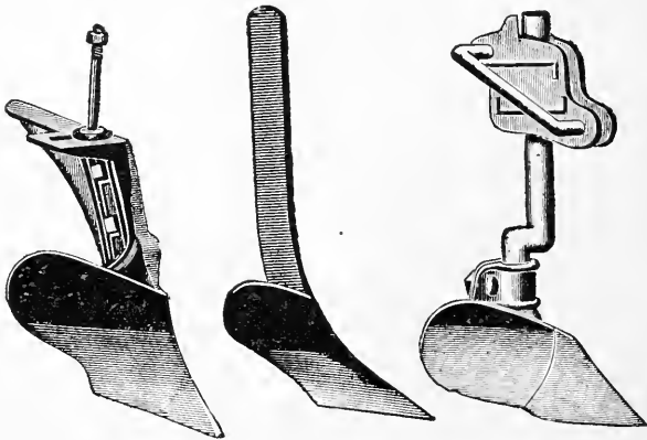
FIG. 42—TYPES OF JOINTERS. THE TWO AT THE LEFT ARE MADE OF STEEL; THE ONE AT THE RIGHT IS A CHILLED IRON JOINTER WITH AN ADJUSTABLE SHANK
