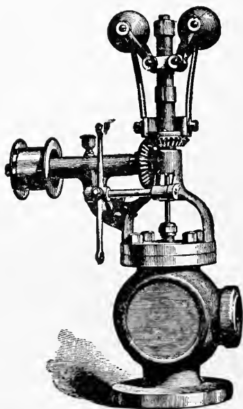
FIG. 271—THROTTLING GOVERNOR
