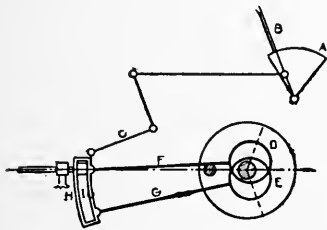
FIG. 260—PRINCIPLE OF STEPHENSON LINK MOTION
