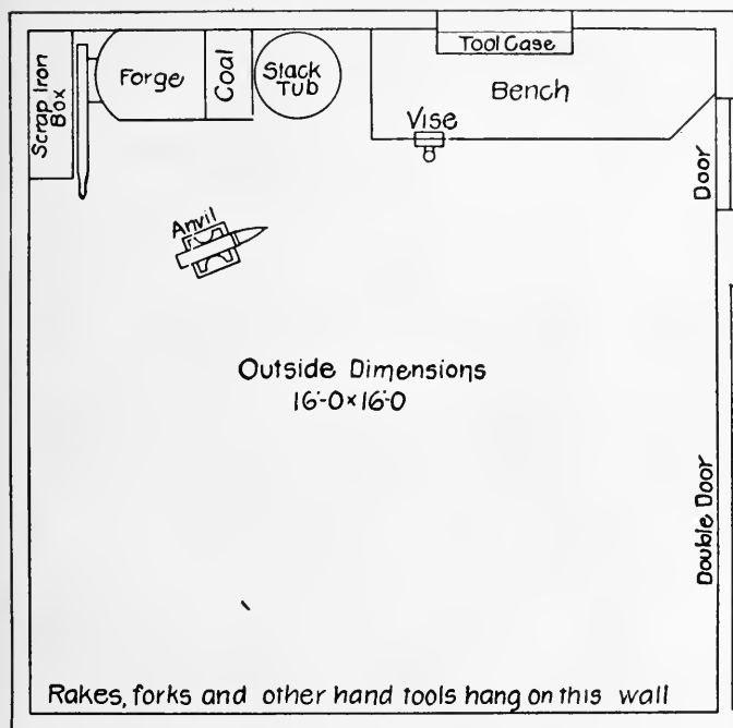
FIG. 376—ARRANGEMENT OF A LARGE SHOP
