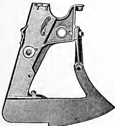
FIG. 94—THE STUB-RUNNER FURROW OPENER
