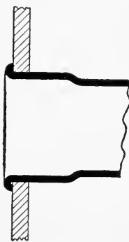
FIG. 241—FLUE EXPANDED WITH DUDGEON EXPANDER
