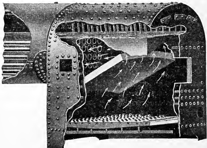
FIG. 219—OPEN-BOTTOM FIRE-BOX BOILER
