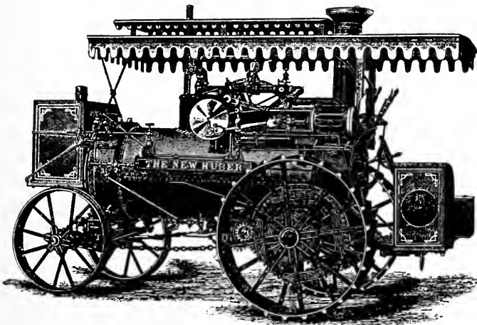
FIG. 324—UNDER-MOUNTED ENGINE
