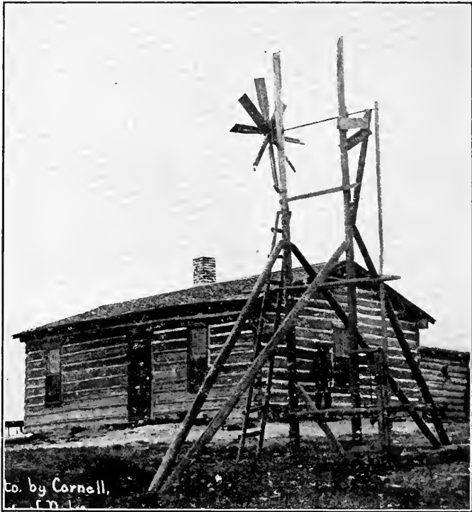
FIG. 204—MOCK TURBINE WINDMILL
