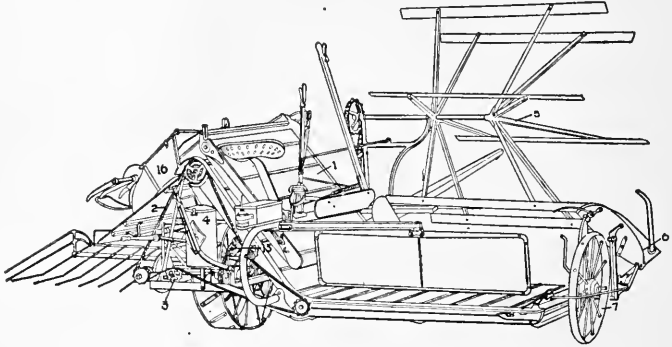
FIG. 110—A MODERN SELF-BINDING HARVESTER OR BINDER
