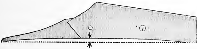
FIG. 48—THE SUCTION OF WALKING PLOWS SOMEWHAT EXAGGERATED
