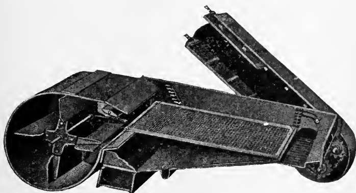
FIG. 161.—FAN, SHOE, AND CHAFFER
