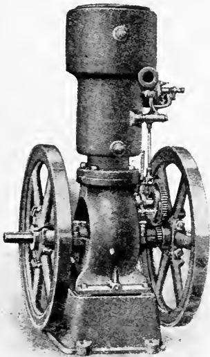
FIG. 311A—OPEN-JACKET SYSTEM OF COOLING
