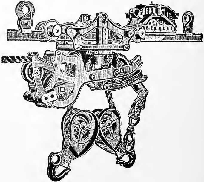
FIG. 141—A DOUBLE-CARRIAGE REVERSIBLE SLING CARRIER. DESIGNED FOR HEAVY SERVICE
