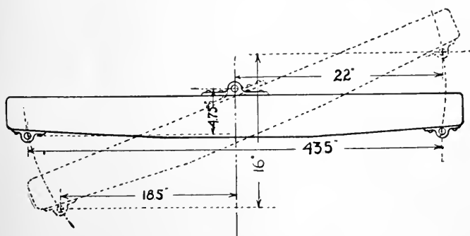
FIG. 2—WAGON EVENER IN OUTLINE. SHOWING THE ADVANTAGE THE LEADING HORSE HAS WHEN THE CLEVIS HOLES ARE NOT A STRAIGHT LINE
