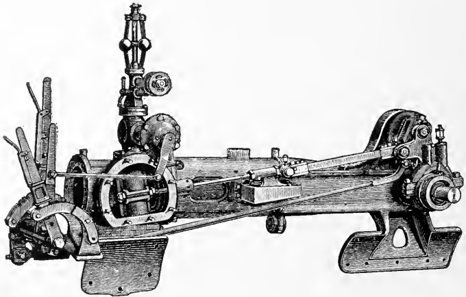
FIG. 261—WOOLF REVERSE GEAR
