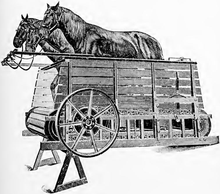
FIG. 200—TREAD POWER FOR THREE HORSES
