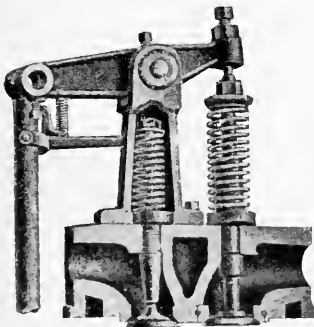
FIG. 298—INLET VALVE LOCK
