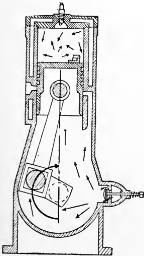
FIG. 287—SUCTION, COMPRESSION AND IGNITION STROKE OF TWO-CYCLE ENGINE
