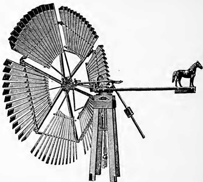
FIG. 209.—SECTIONAL WHEEL WITH NO RUDDER
