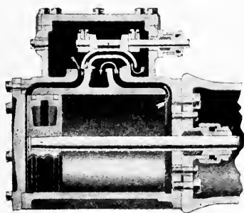
FIG. 252—DOUBLE-PORTED VALVE
