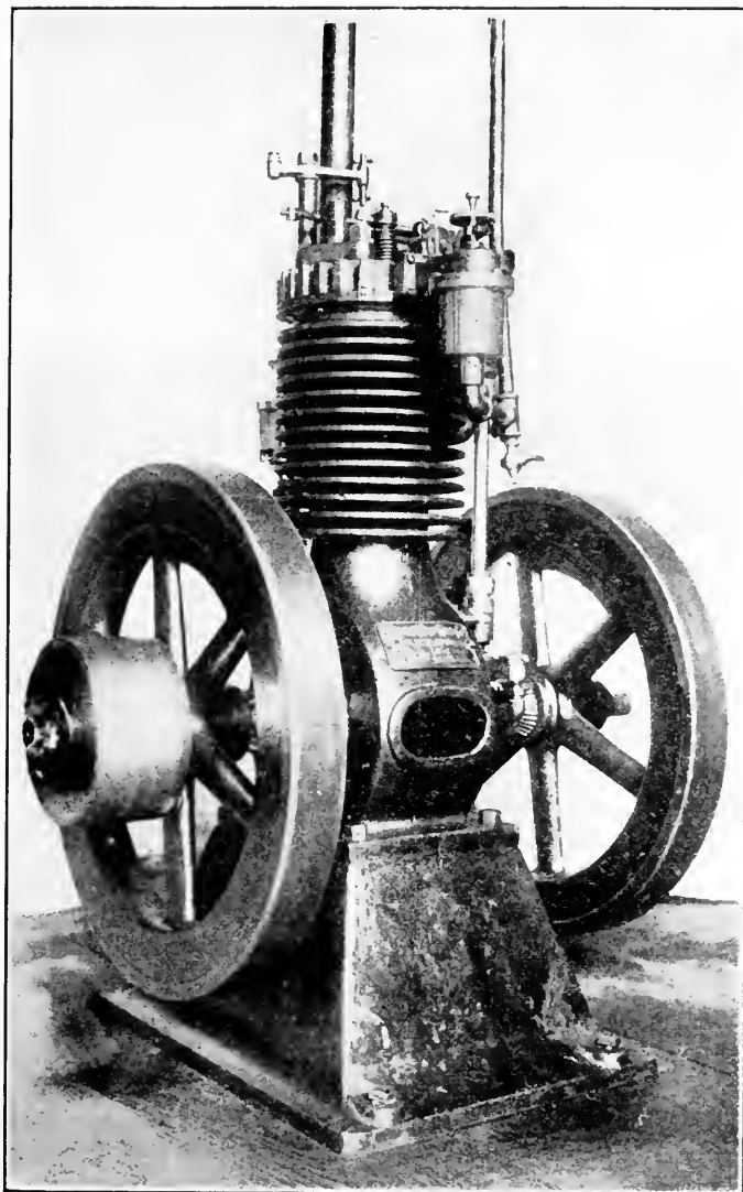
FIG. 310—AIR-COOLED ENGINE
