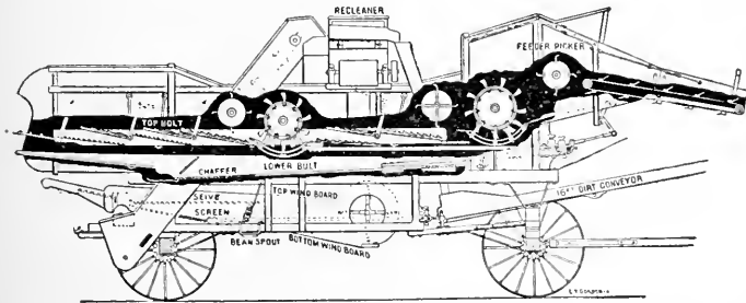
FIG. 165—SECTION OF A PEA AND BEAN THRESHER WITH TWO CYLINDERS
