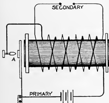
FIG. 374—PRINCIPLE OF THE INDUCTION COIL
