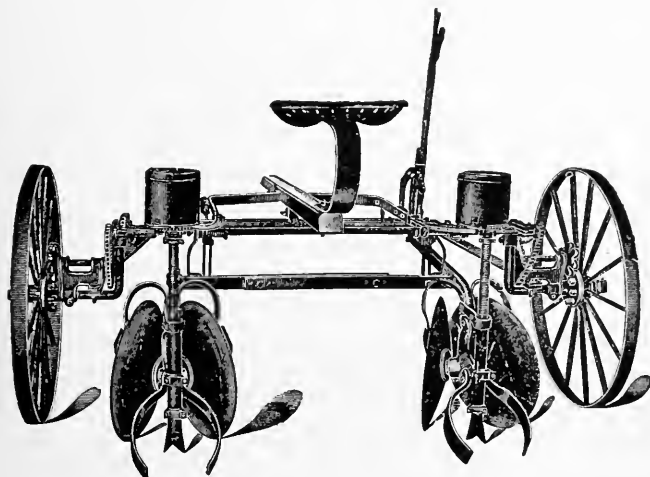
FIG. 102—A LOOSE-GROUND LISTER. DISK FURROW OPENERS MAY BE USED ON PLANTER FOR THE SAME PURPOSE
