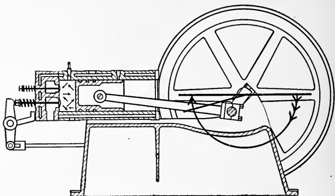
FIG. 282—COMPRESSION AND IGNITION STROKE OF FOUR-CYCLE ENGINE
