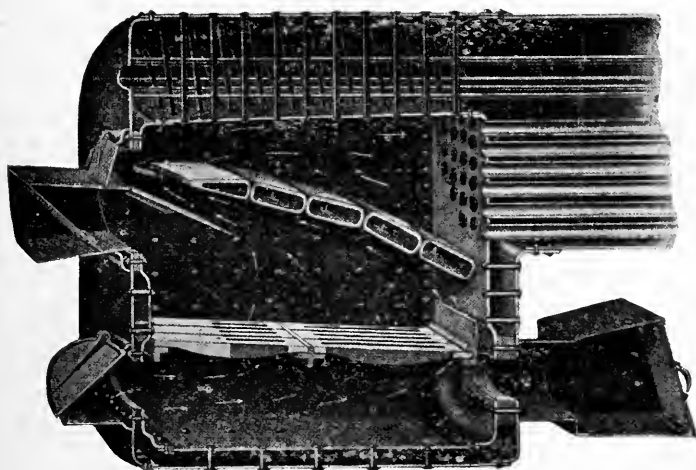
FIG. 224.—STRAW BURNER DIRECT-FLUE BOILER
