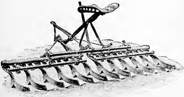
FIG. 51—A CURVED KNIFE-TOOTH HARROW OR PULVERIZER
