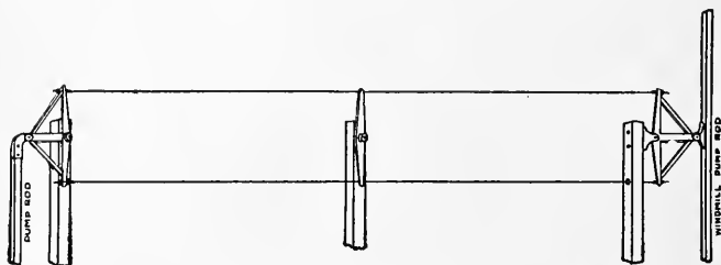
FIG. 23—THE TRANSMISSION OF THE POWER OF A WINDMILL TO A PUMP AT A DISTANCE BY MEANS OF TRIANGLES AND WIRES
