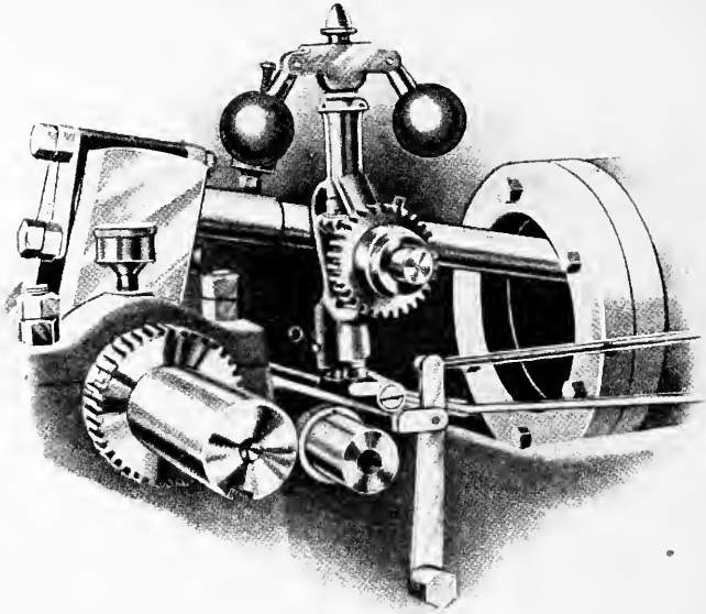
FIG. 300—BALL GOVERNOR
