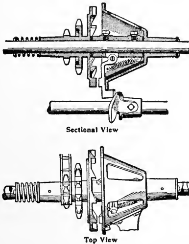
FIG. 92—THE SEED-SHAFT CLUTCH WHICH IS THROWN IN GEAR BY THE CHECK WIRE. THE POWER TO DRIVE THE SEED SHAFT THEN COMES FROM THE MAIN AXLE, NOT THE CHECK WIRE
