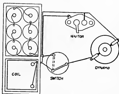
FIG. 309—WIRING SYSTEM FOR BATTERIES AND DYNAMOS
