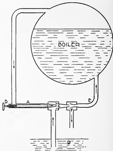
FIG. 229—PRINCIPLE OF THE INJECTOR
